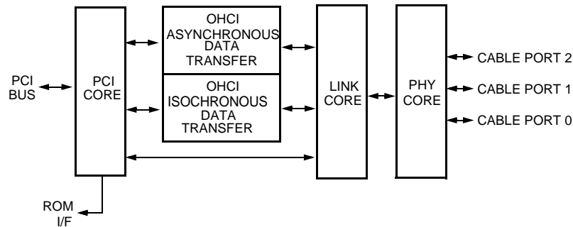
Figure 1. FW323 07 NV129 1394a Mode Block Diagram
