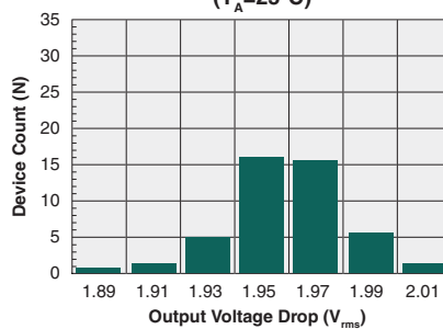
Typical On-State Output Forward Voltage Distribution ( T_A=25^\circ\text{C} )
