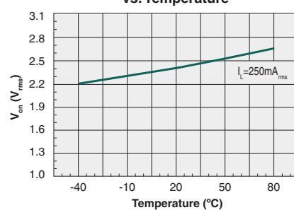
Typical Output Voltage Drop vs. Temperature
