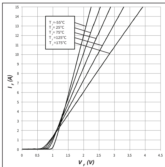
Figure 1. Forward Characteristics
