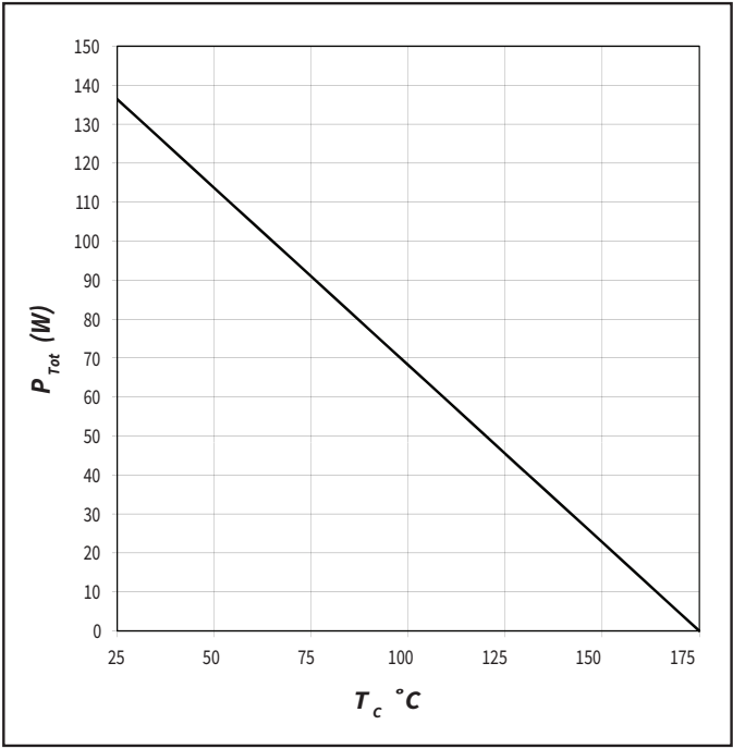
Figure 4. Power Derating
