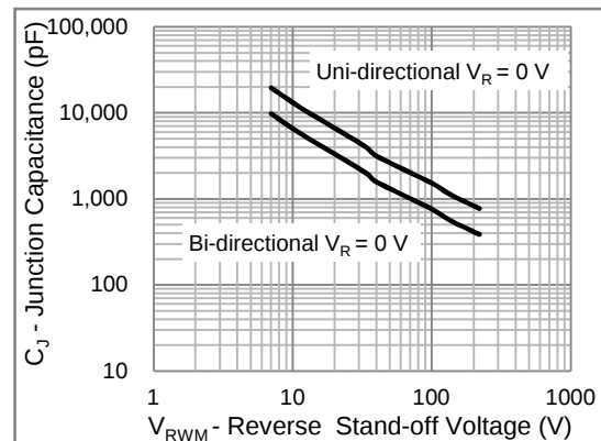
Fig.4 Typical Capacitance
