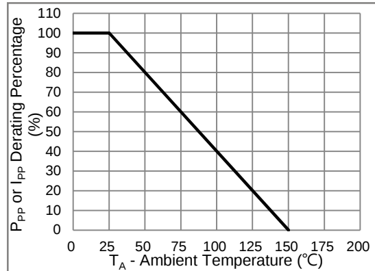
Fig.2 Derating Curve
