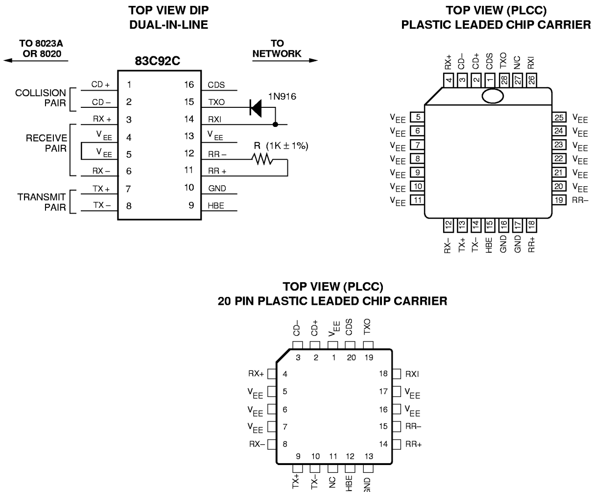
Figure 2. 83C92C Ethernet Transceiver Pin Configuration
