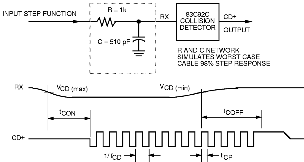
Figure 6. Collision Timing
