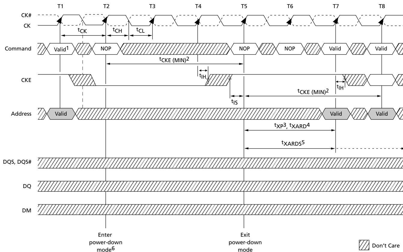
Figure 70: Power-Down
