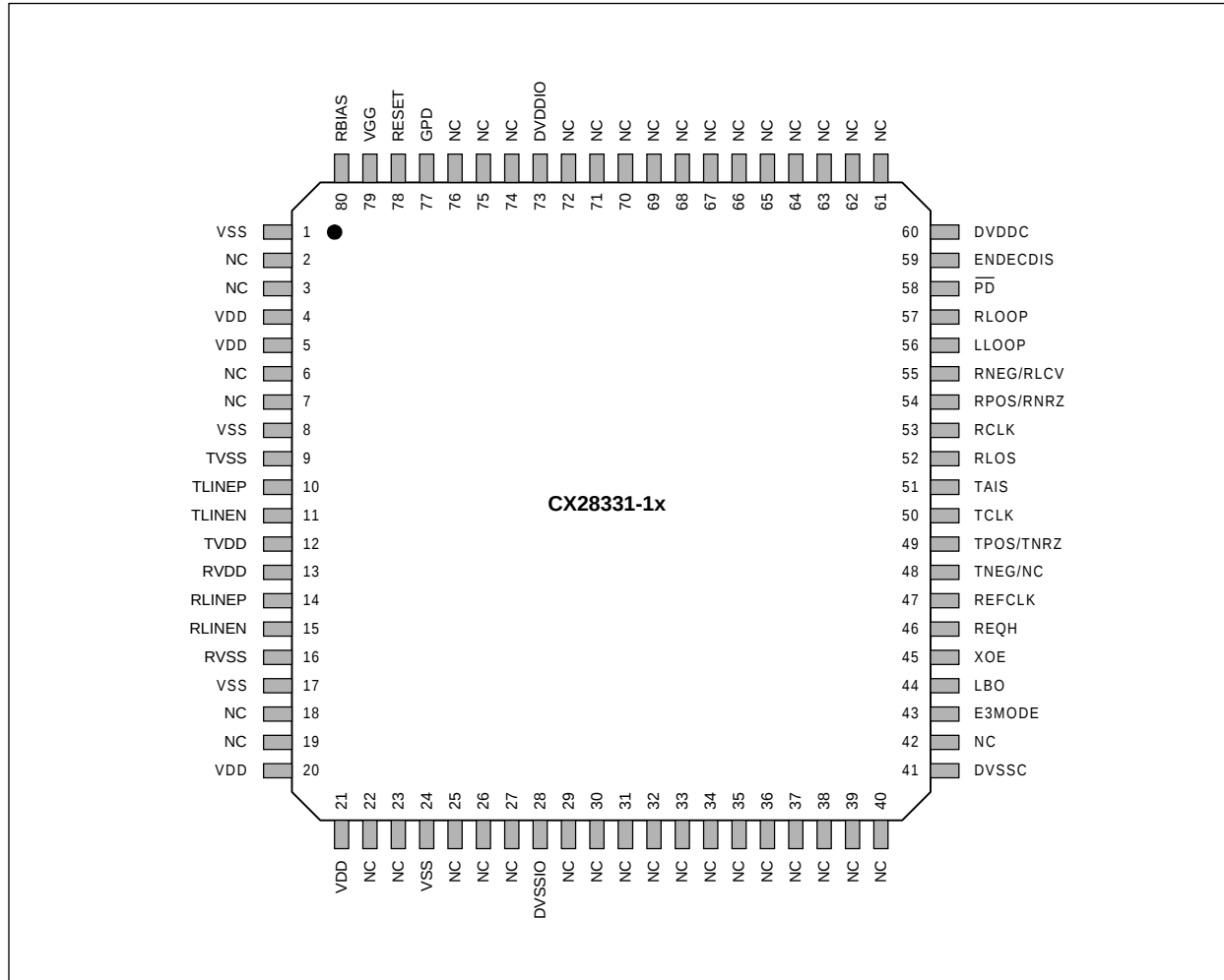
Figure 1-1. CX28331-1x Pin Diagram
