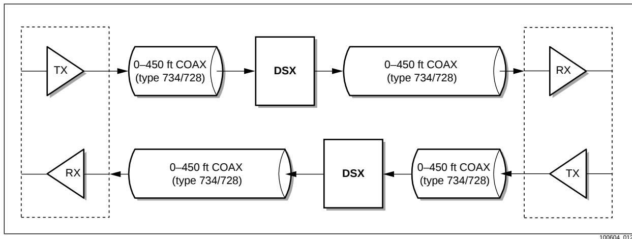
Figure 2-1. Typical Application Of Single CX2833i Channel
