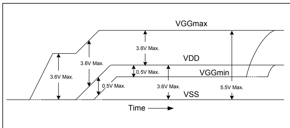
Figure C-1. Power-up sequence of VGG and VDD.
