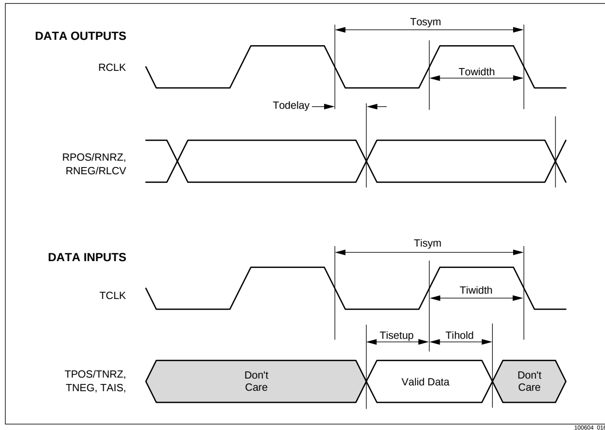
Figure 2-13. Timing Diagram
