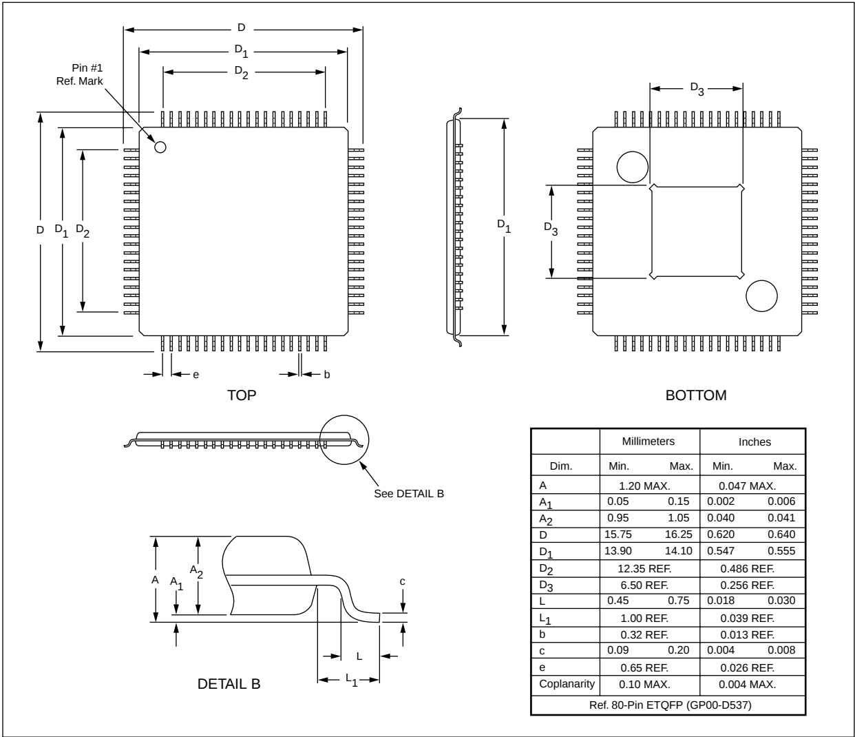
Figure 2-12. CX2833i-1x Mechanical Drawing (80-Pin)—Dimensions
