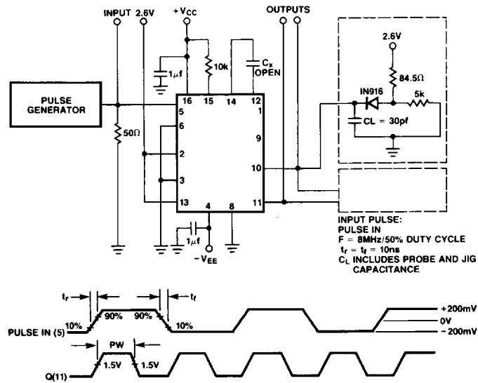
Figure 1. Minimum Output Pulse Width ( C_{X2} = \text{OPEN} )
