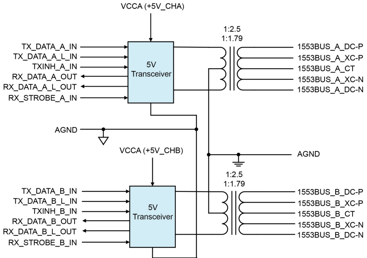
Figure 2. BU-67402 Block Diagram
