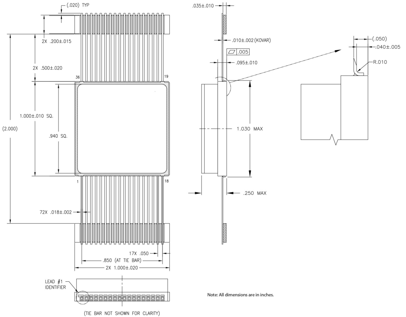
Figure 5. BU-67402 Mechanical Outline – SPACE-PHY 36-pin Flat Package
