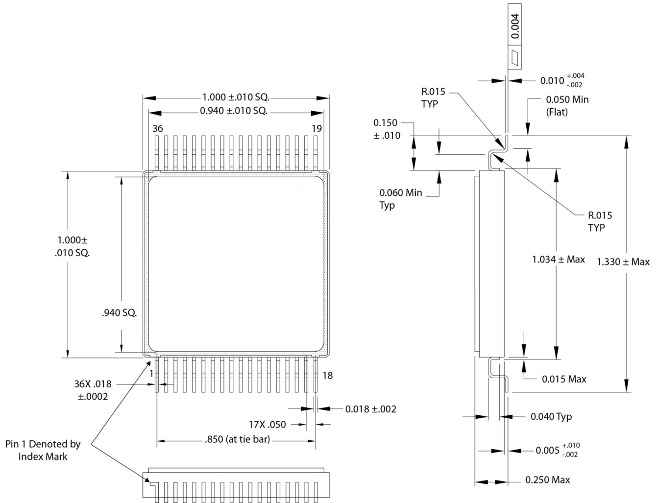
Figure 6. BU-67402 Mechanical Outline – SPACE-PHY 36-pin Gull Wing Package
