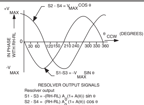
FIGURE 2B. RESOLVER OUTPUT SIGNALS
