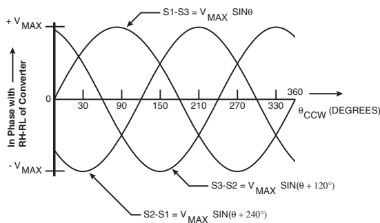
FIGURE 2A. SYNCHRO OUTPUT SIGNALS
