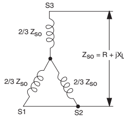
FIGURE 3. Z_{SO} MEASUREMENT
