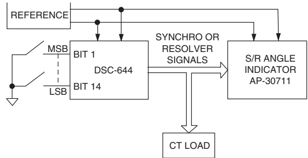
FIGURE 5. ACCURACY TEST CIRCUIT
