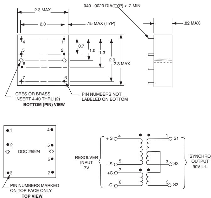
TRANSFORMER CONNECTIONS
