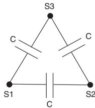
FIGURE 4. DELTA TUNING CONFIGURATION
