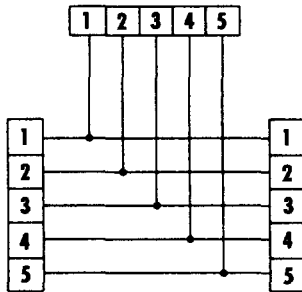
WIRING DIAGRAM
