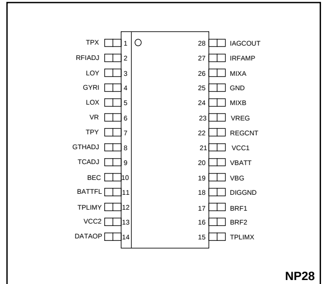
Fig.1 Pin connections
