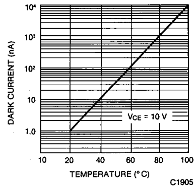
Fig. 4. Collector Dark Current vs. Ambient Temperature
