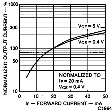
Fig. 1. Normalized Output Current vs. Input Current
