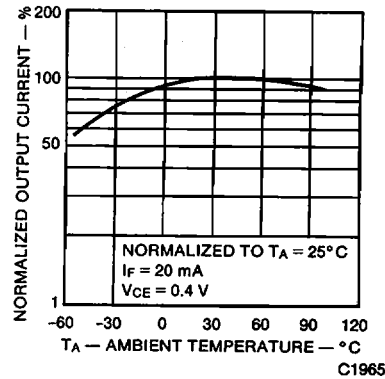
Fig. 2. Normalized Output Current vs. Ambient Temperature
