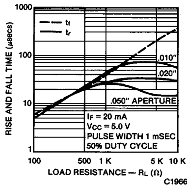
Fig. 5. Rise and Fall Time vs. Load Resistance
