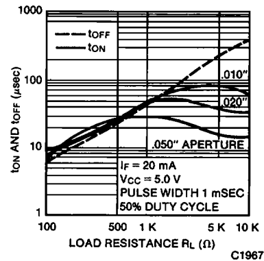
Fig. 6. Turn-on and Turn-off Time vs. Load Resistance
