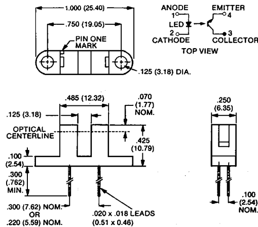
Package 6 Dimensions
