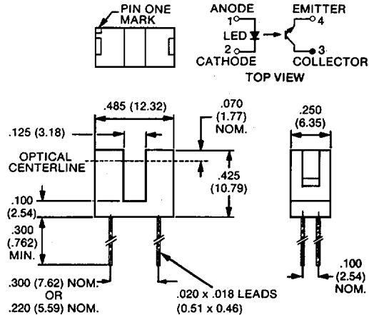
Package 7 Dimensions
