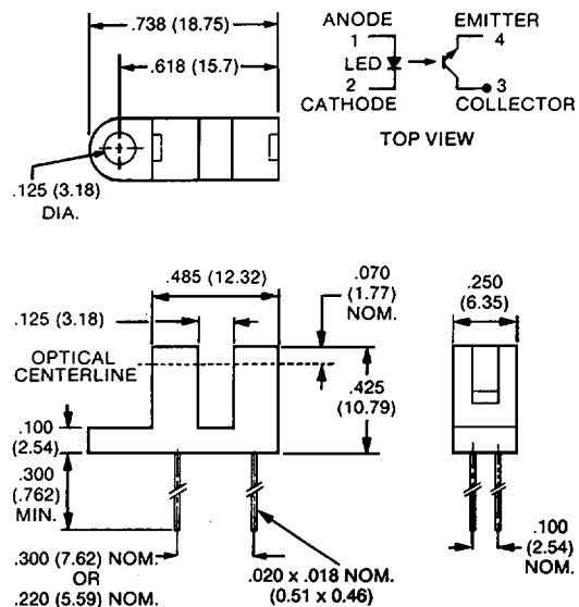
Package 7 Dimensions
