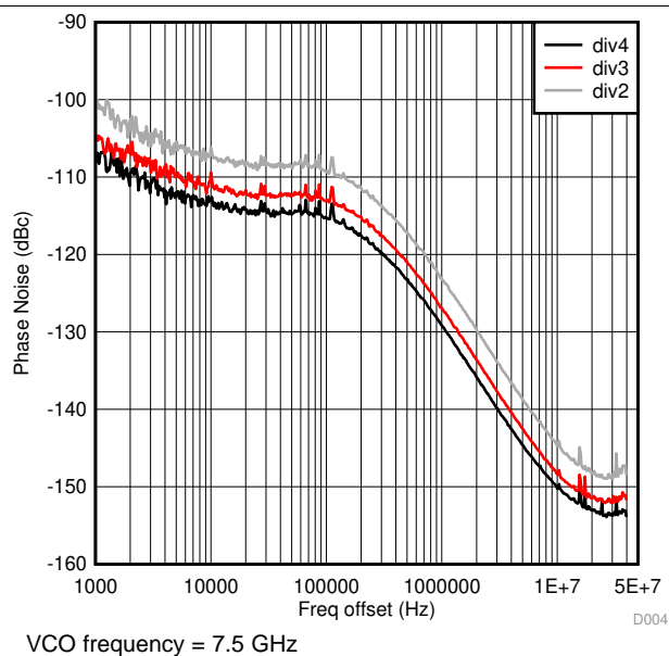
Figure 20. DAC38RF89 VCO1 Output Clock Phase Noise vs Offset frequency Over Divider Ratio
