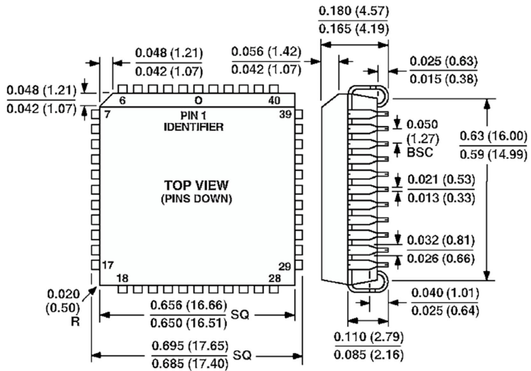
Figure 15: 44 Lead PLCC Mechanical Outline
