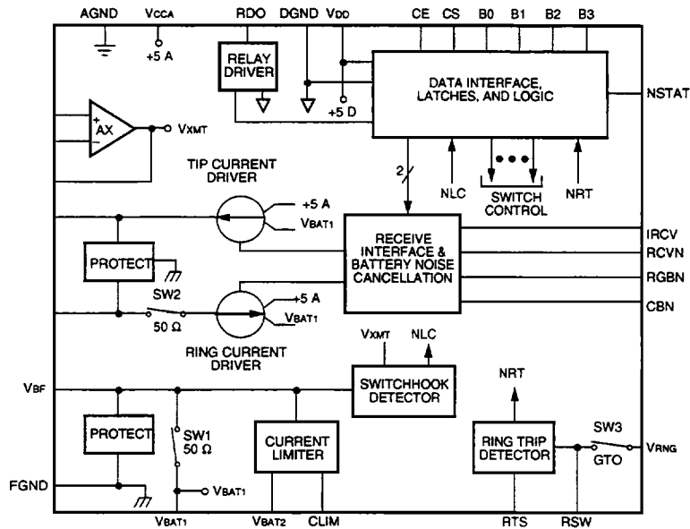
Figure 1. Architectural Diagram
