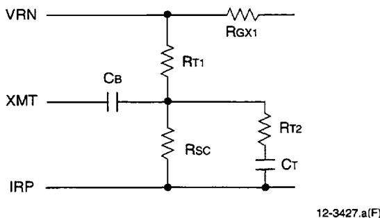
Figure 14. Addition of Resistor R_{sc} from XMT to IRP
