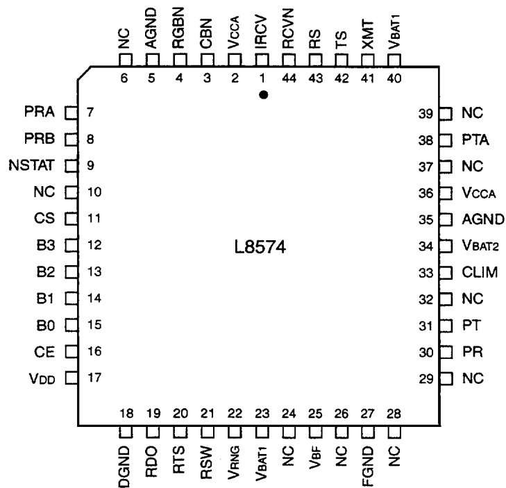
Figure 2. Pin Layout
