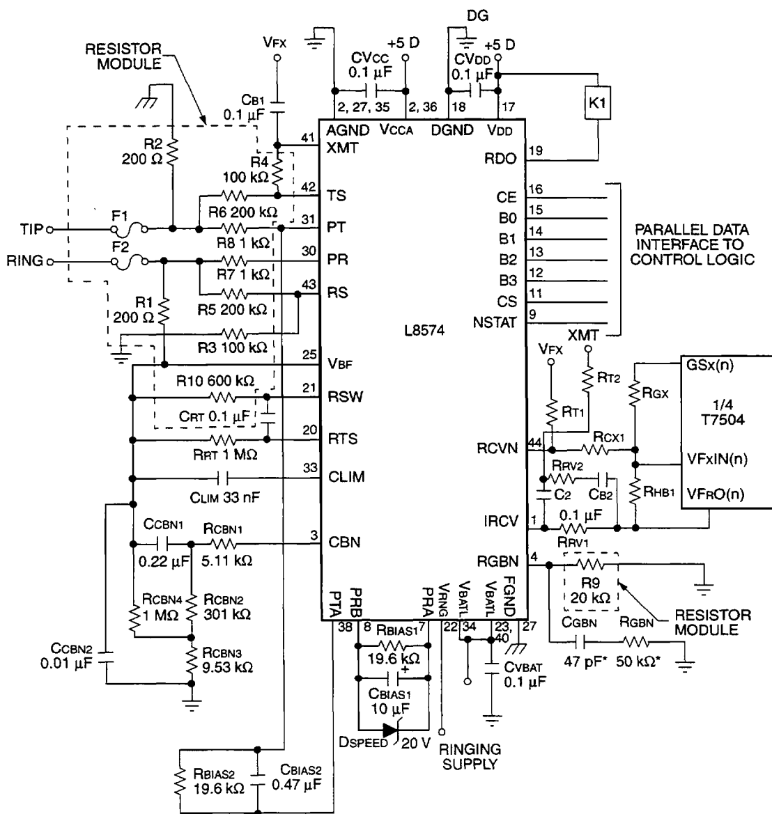
Figure 5. External Components Required
