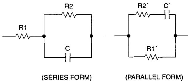
Figure 11. Equivalent Complex Terminations
