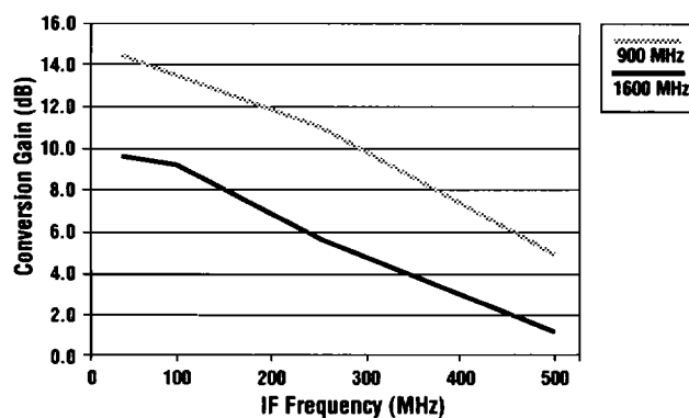
Conversion Gain vs. IF Frequency
