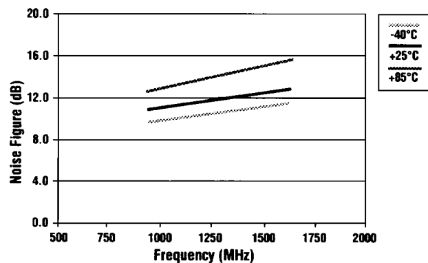
Noise Figure vs. Frequency vs. Temperature
