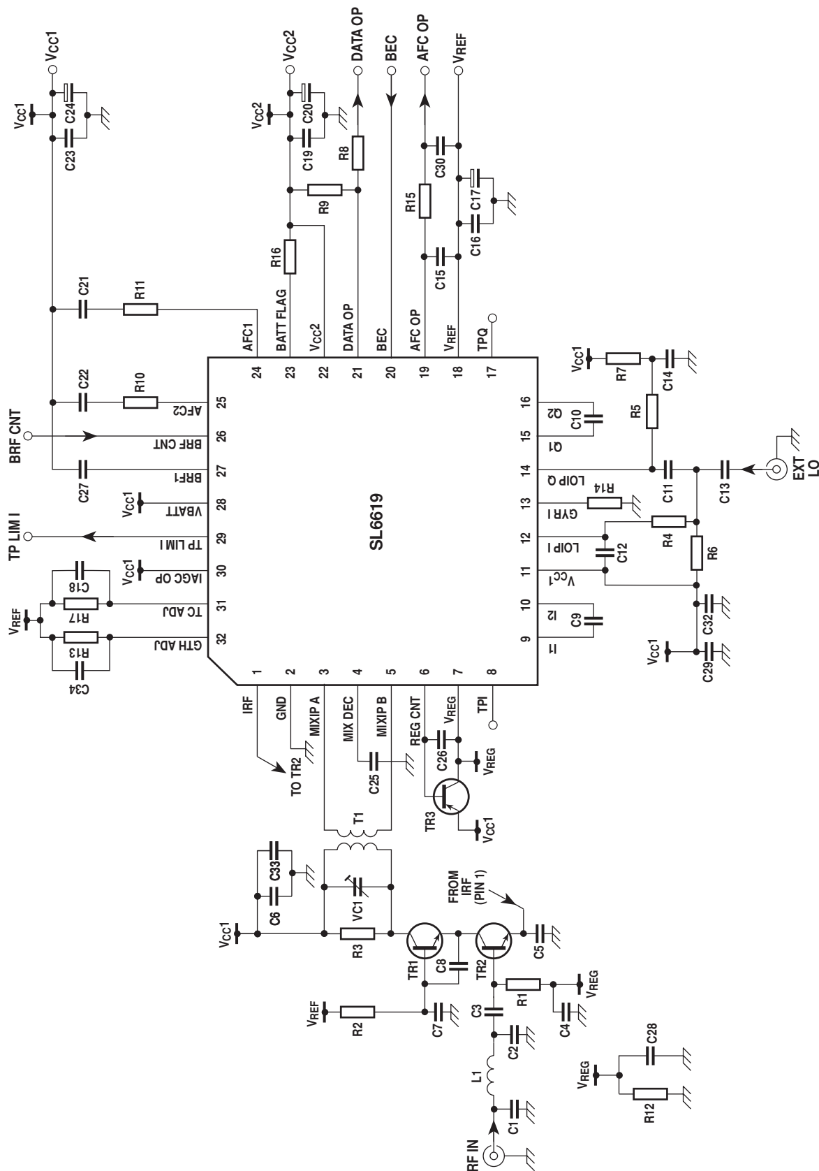
Figure 5 - SL6619 characterisation circuit (see Tables 3 and 4 for component values)
