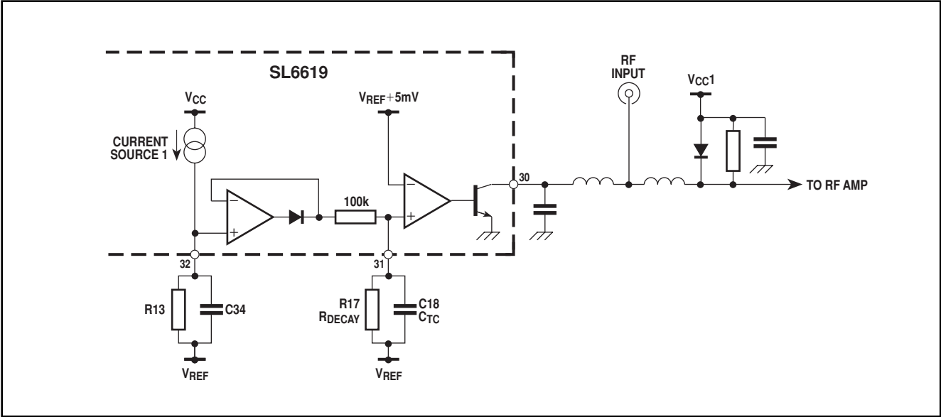
Figure 3 - AGC schematic
