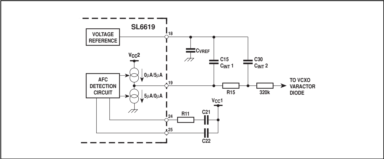
Figure 4 - AFC schematic
