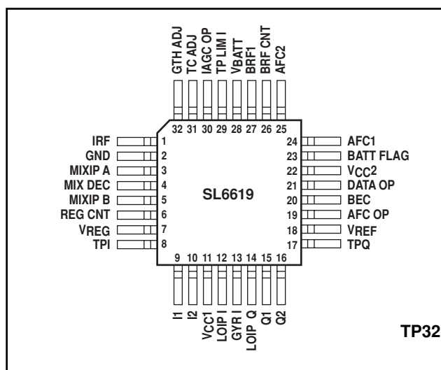
Figure 1 Pin identification diagram (top view). See Table 1 for pin descriptions
