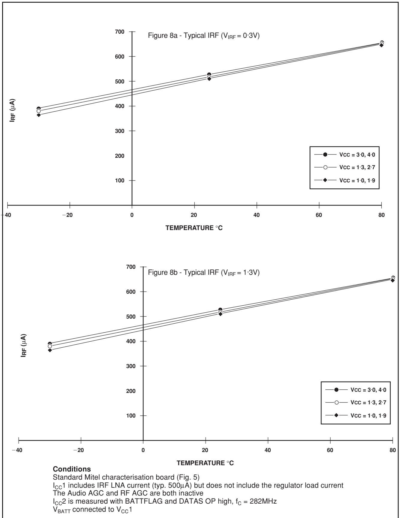
Figure 8 - Typical I_{RF} v. supply and temperature
