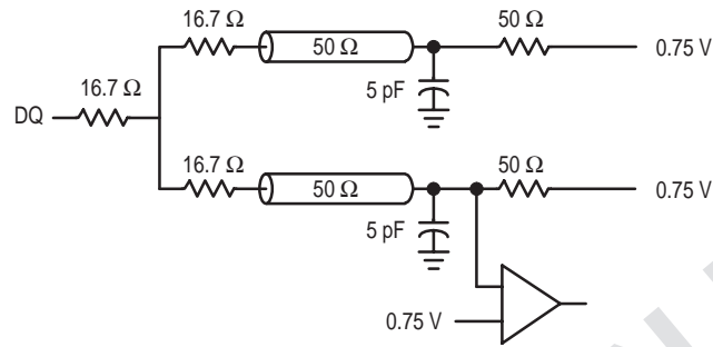
Figure 1. Test Loads
