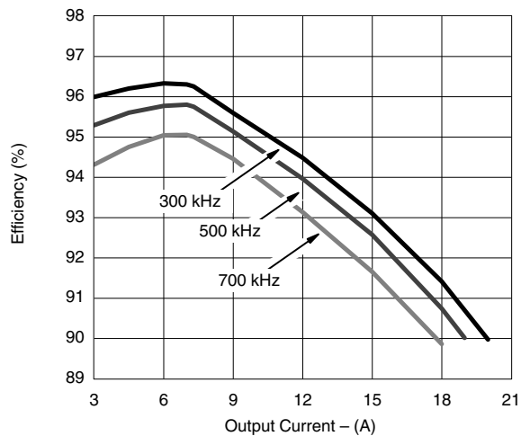
Figure 5. Total Efficiency 5 V IN /2.5 V OUT
