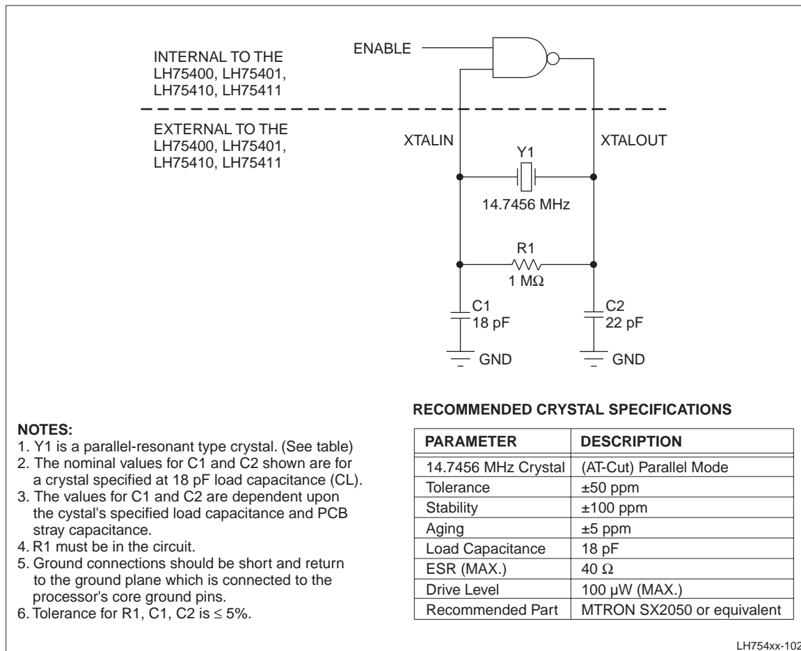
Figure 19. Suggested External Components, 14.7456 MHz Oscillator
