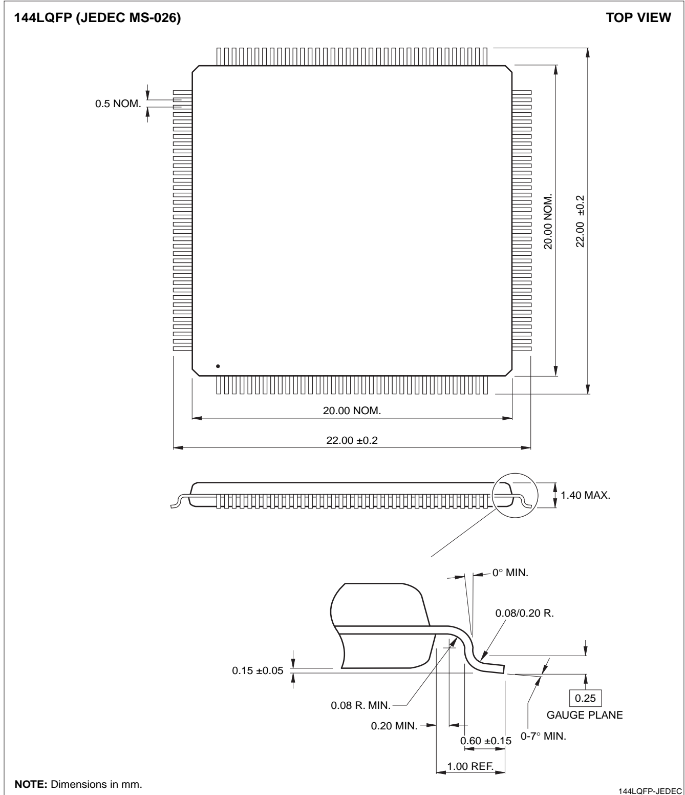
Figure 20. 144-pin LQFP
