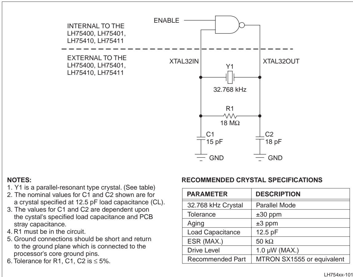
Figure 18. Suggested External Components, 32.768 kHz Oscillator
