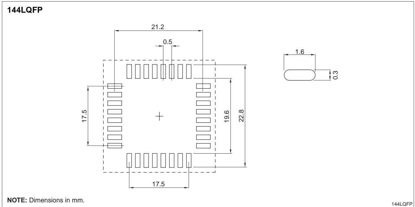
Figure 21. Recommended PCB Footprint
