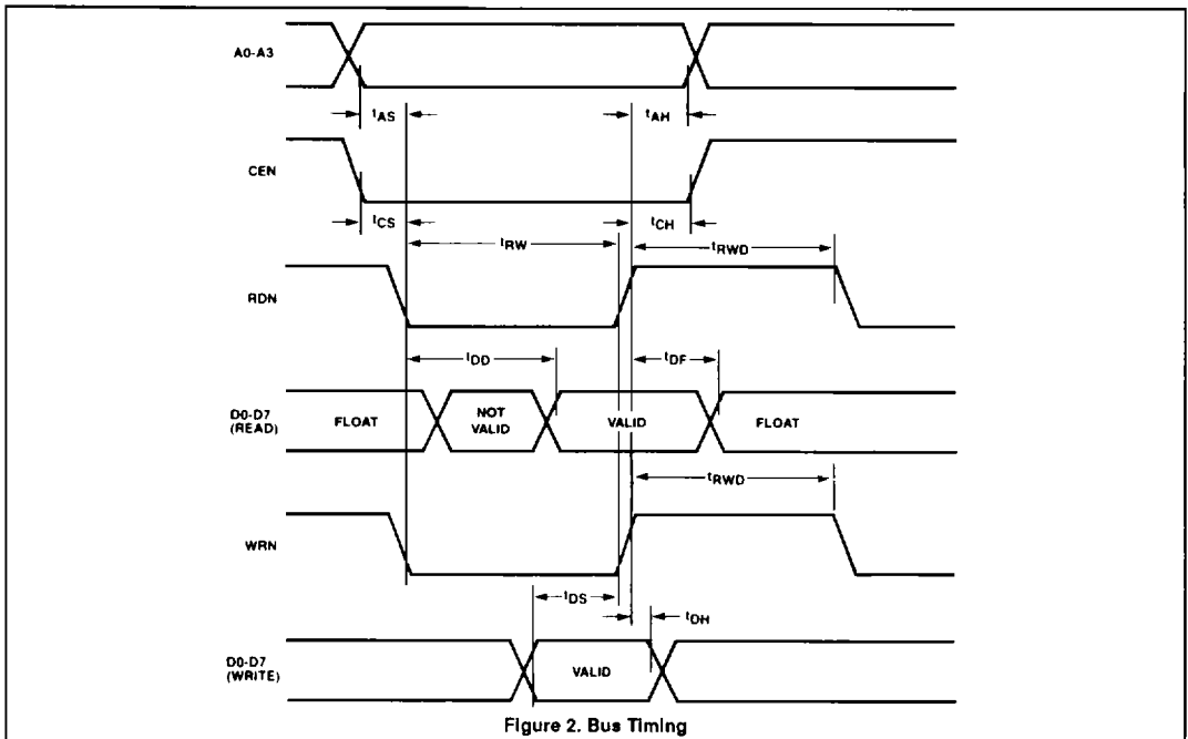
Figure 2. Bus Timing
