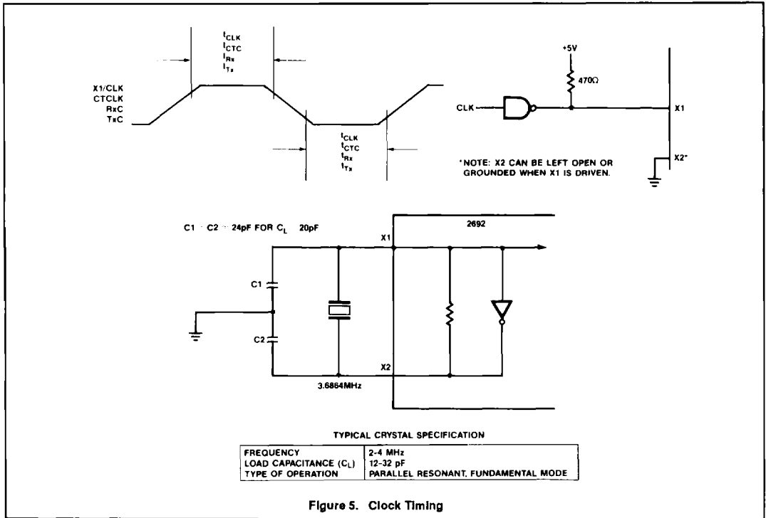
Figure 5. Clock Timing
