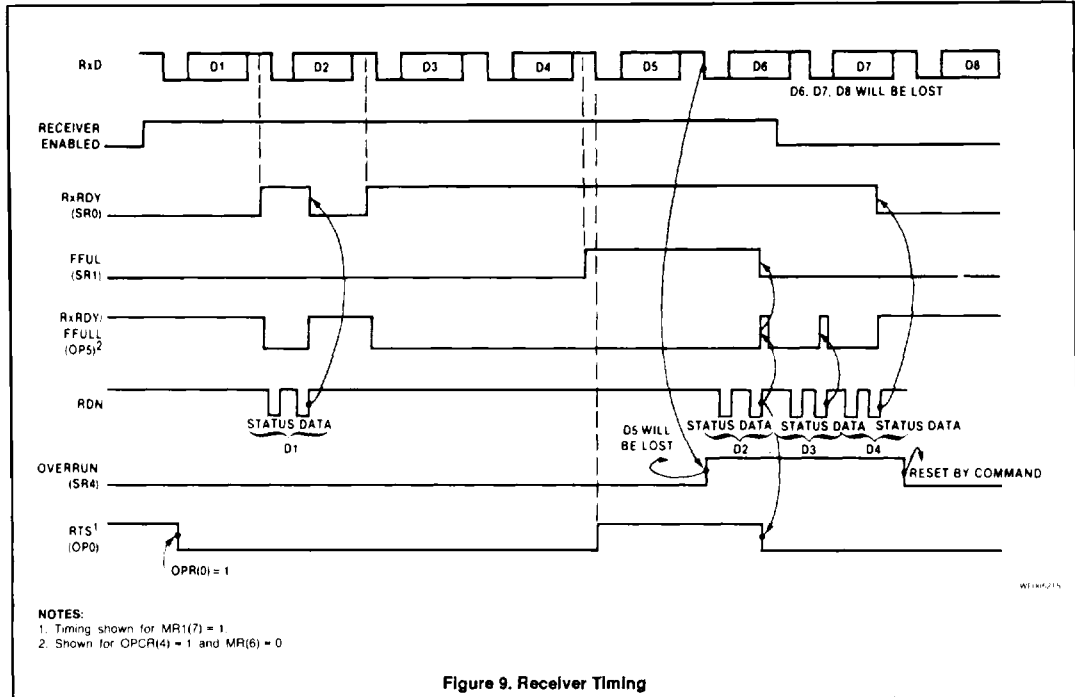
Figure 9. Receiver Timing
