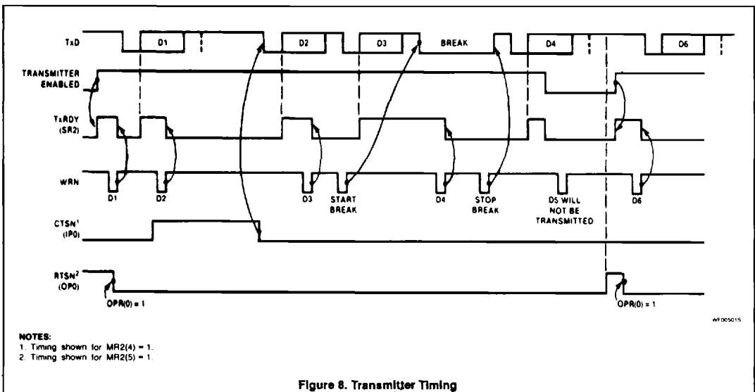
Figure 8. Transmitter Timing
