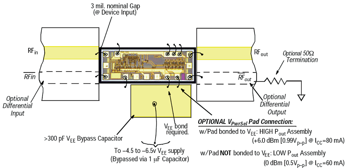
Figure 3. Assembly diagrams
