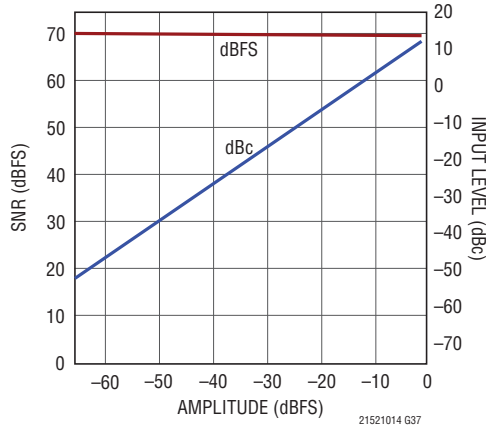
LTC2151-14: SNR vs Input Level, f_{IN} = 71\text{MHz} , 1.5V Range, 210Mpsps
