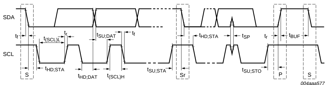
Fig 19. Definition of timing for standard-mode or fast-mode devices on the I 2 C-bus.
