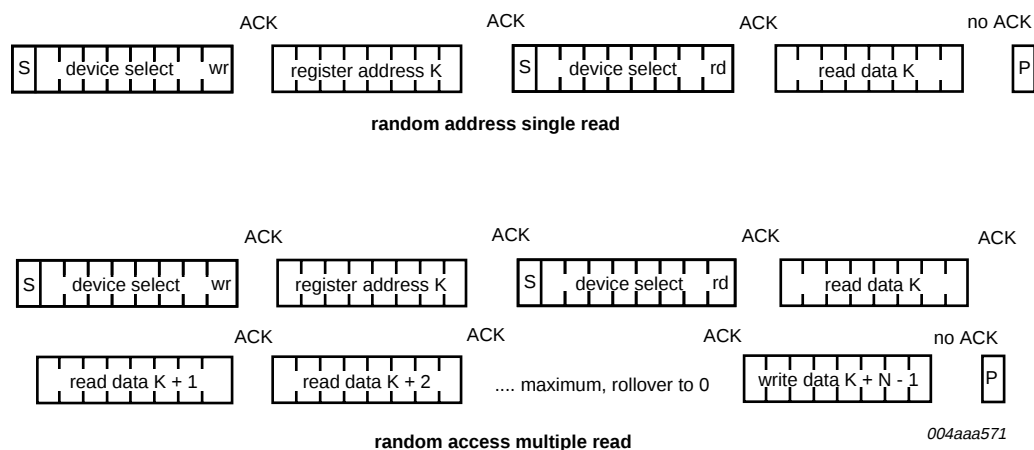
Fig 11. Random address read.
