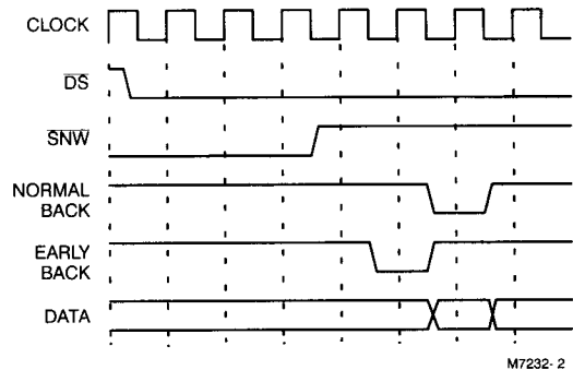
Figure 1. Early and Normal Bus Acknowledge Modes for Reads
