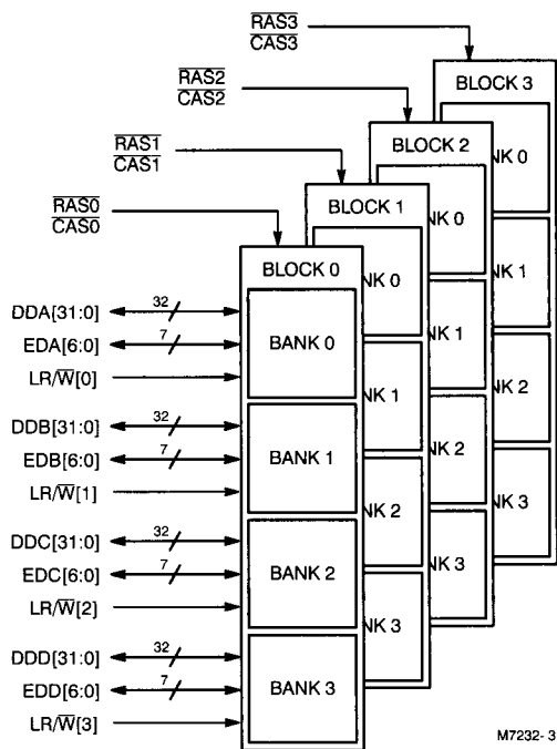
Figure 3. DRAM Configuration for the CYM7232
