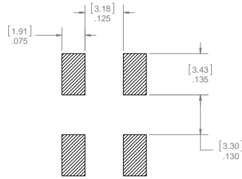
Recommended Pad Outline
