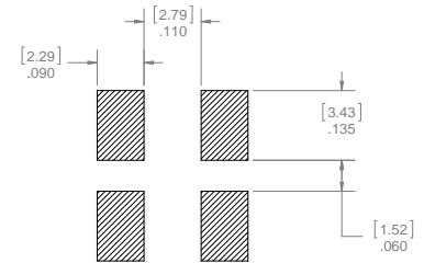
Recommended Pad Outline
