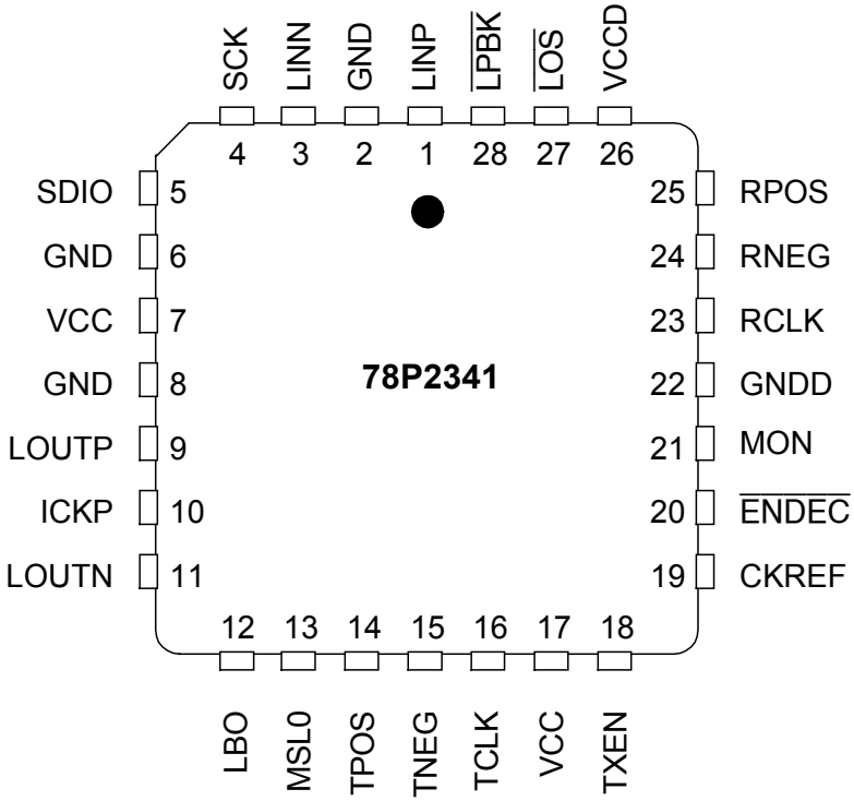
28-pin PLCC
