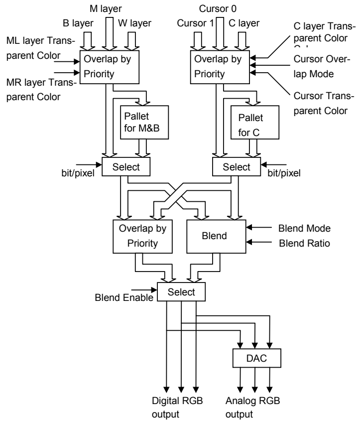
Fig. 5.4 Display data processing flow
