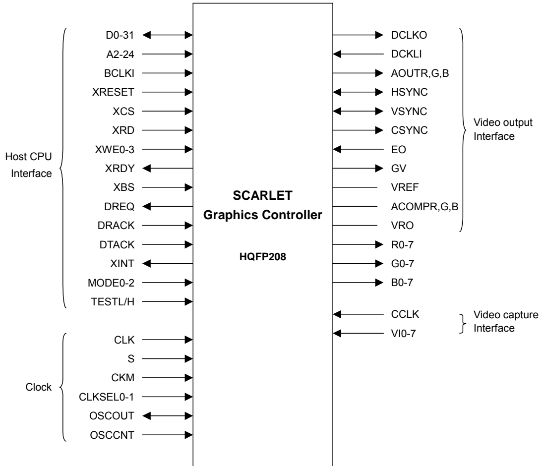
Fig. 2.1 SCARLET Signals
