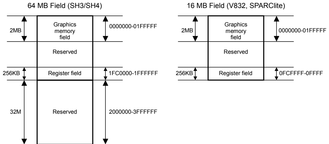
Fig. 4.1 Memory Map
