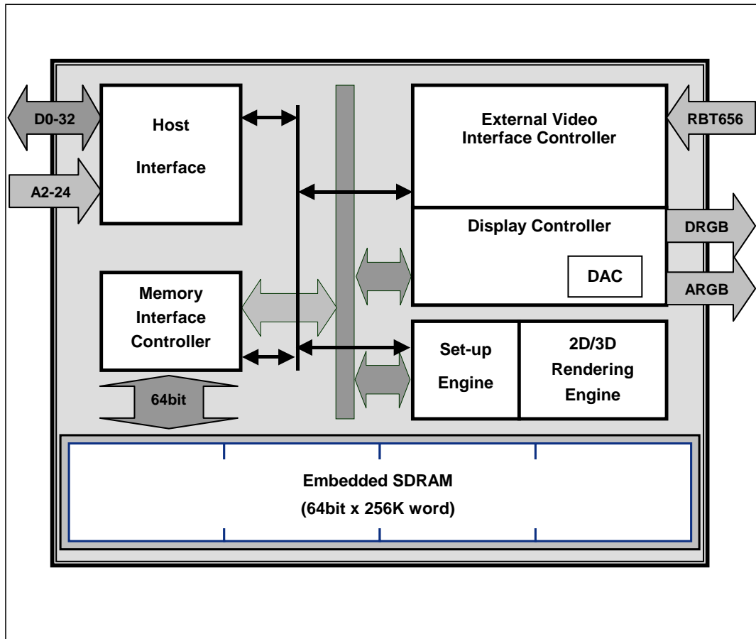
Fig.1.2 SCARLET Block Diagram (TBD)
