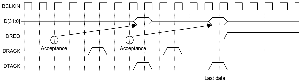
Fig. 11.14 SH4 Single-address DMA Transfer End Timing
