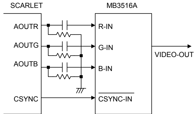
Fig. 5.5 Example of NTSC Encoder Connection
