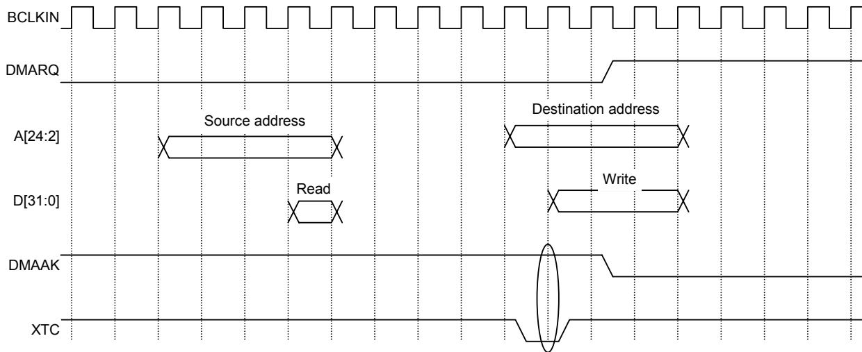
Fig. 11.16 V832 DMA Transfer End Timing
