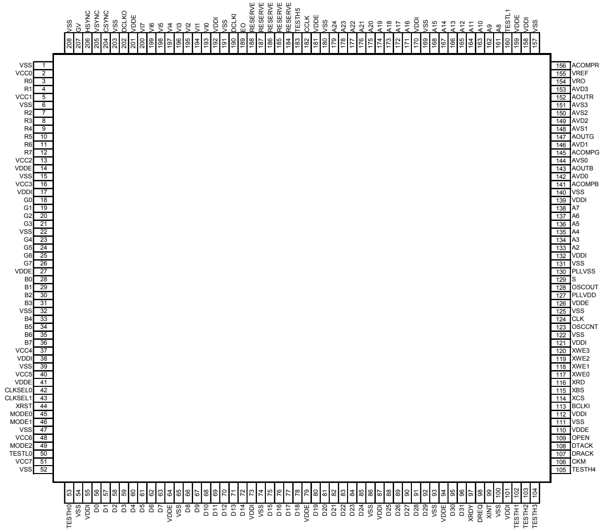
Fig. 2.2 SCARLET Pin Assignment
