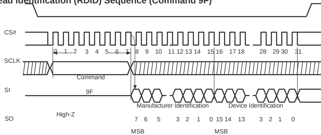
Figure 3. Read Identification (RDID) Sequence (Command 9F)
