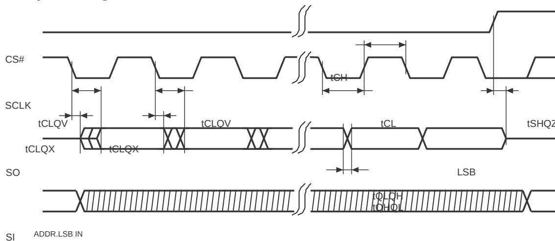
Figure 11. Output Timing
