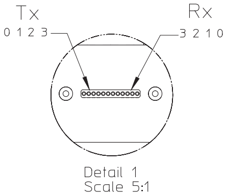
Figure 17. Package Outline for HFBR-779BE and HFBR-789BE (dimensions in mm)
