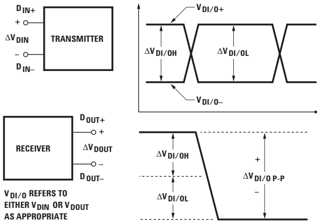
Figure 8. Differential signals.
