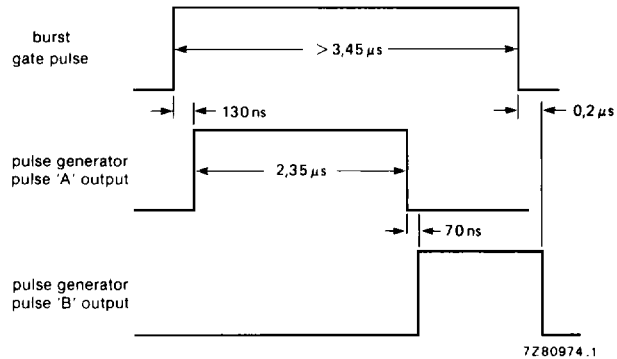
Fig. 2 Burst gate timing pulse generation.
