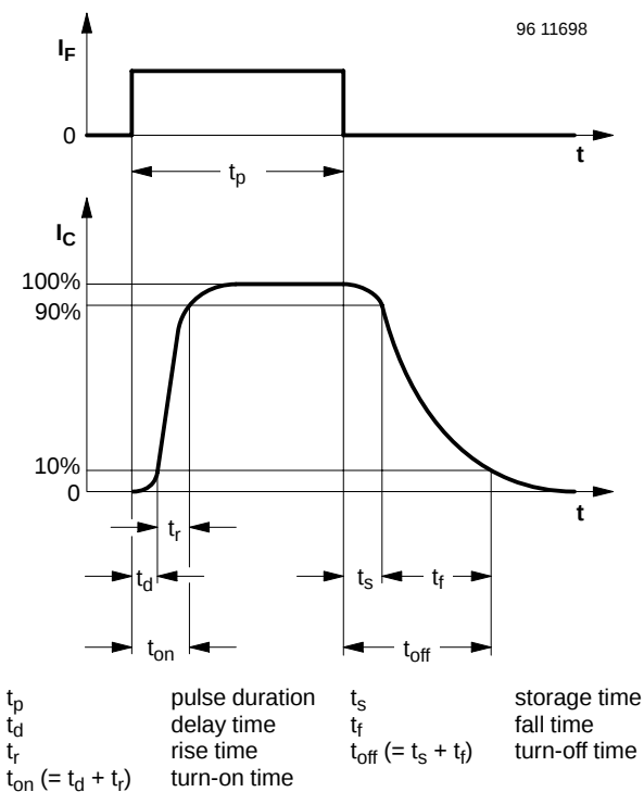
Figure 2. Switching times
