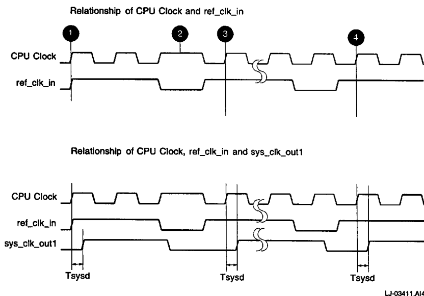
Figure 18 ref_clk System Timing
