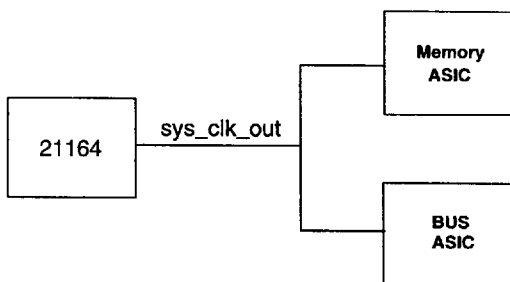
Figure 7 21164 Uniprocessor Clock
