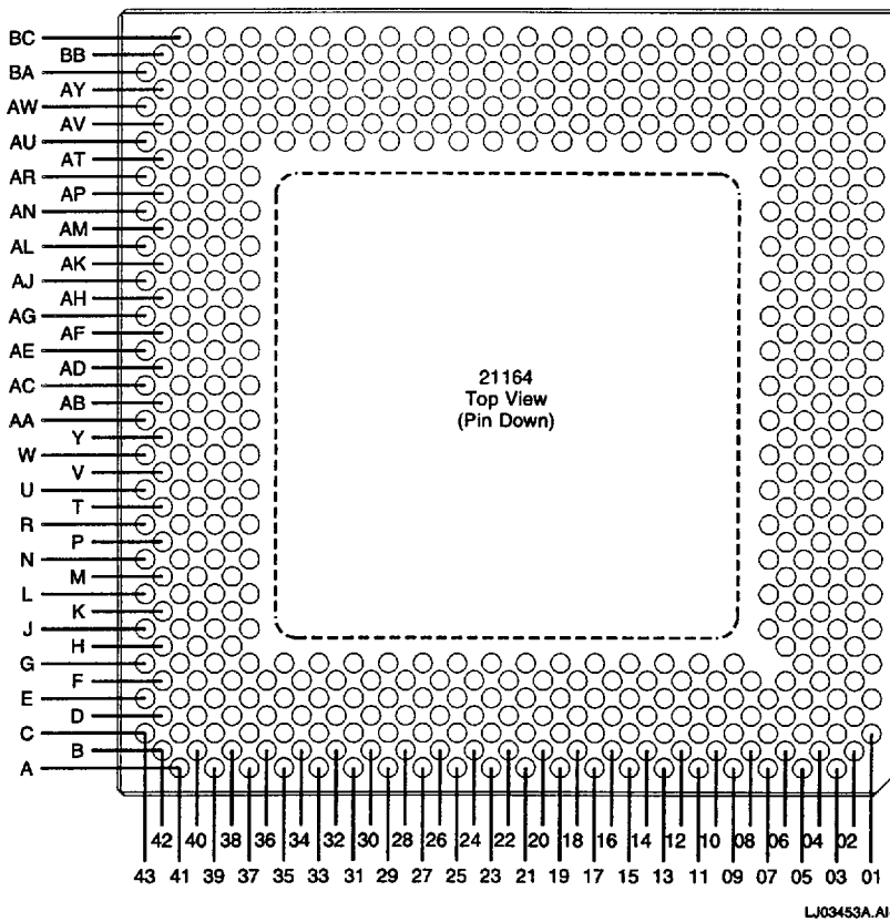
Figure 3 21164 Top View (Pin Down)
