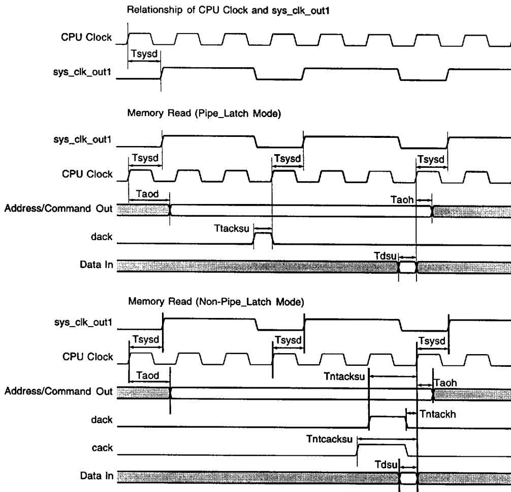
Figure 17 sys_clk System Timing
