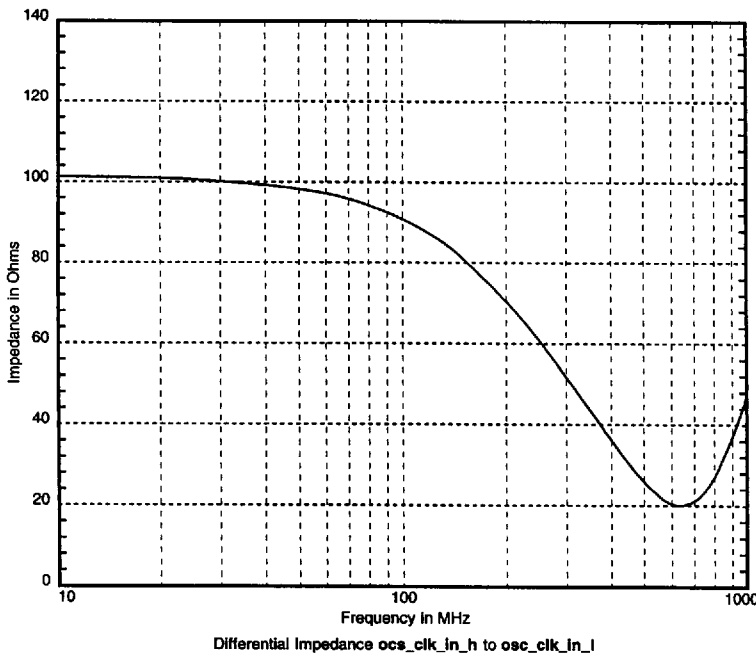
Figure 14 Impedance vs Clock Input Frequency
