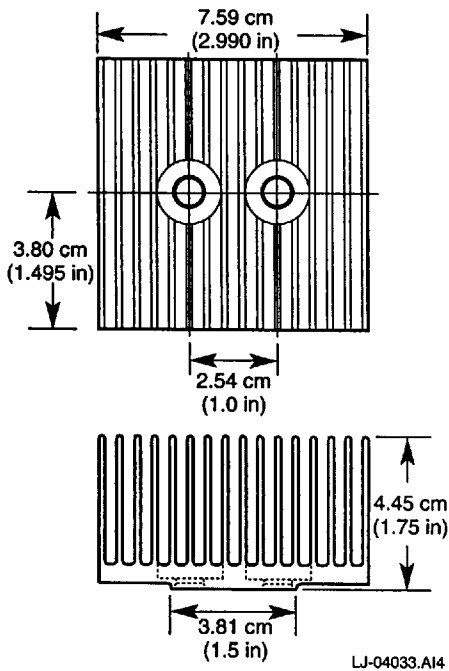
Figure 23 Type 2 Heat Sink
