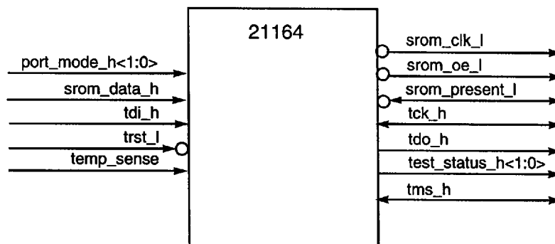
Figure 12 21164 Test Signals
