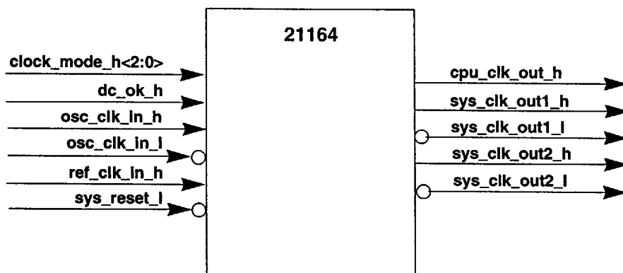
Figure 6 21164 Clock Signals
