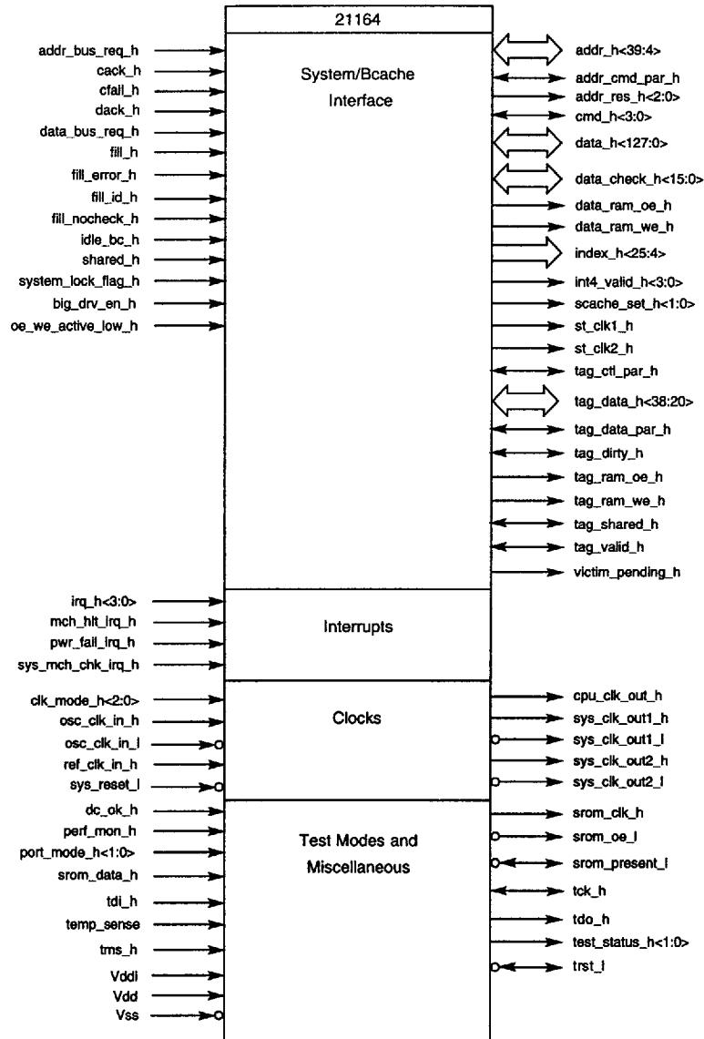
Figure 5 21164 Microprocessor Logic Symbol
