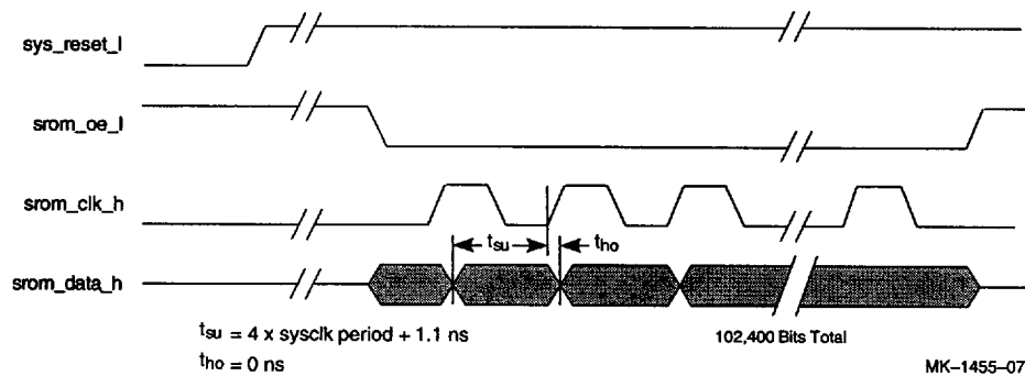
Figure 21 Serial ROM Load Timing
