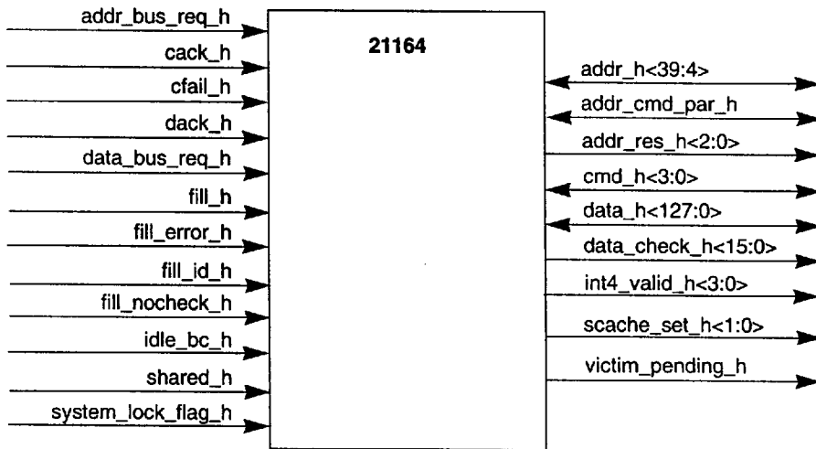
Figure 10 21164 System Interface Signals
