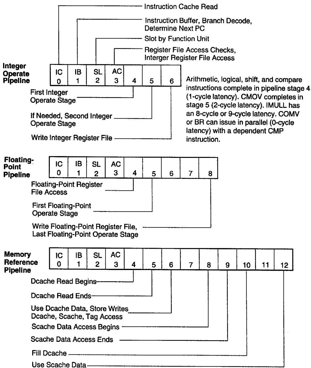
Figure 2 Instruction Pipeline Stages
