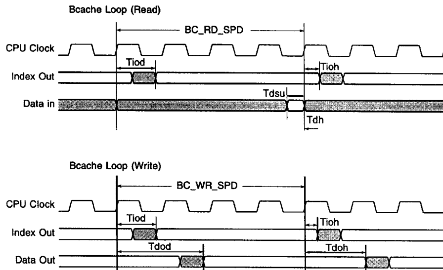
Figure 16 Bcache Timing
