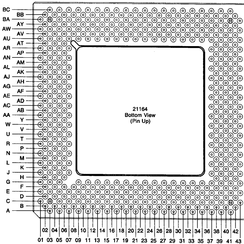
Figure 4 21164 Bottom View (Pin Up)
