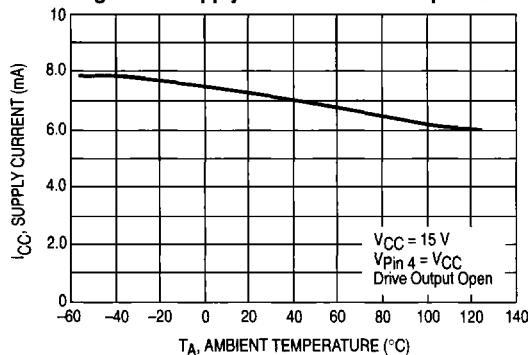
Figure 28. Supply Current versus Temperature
