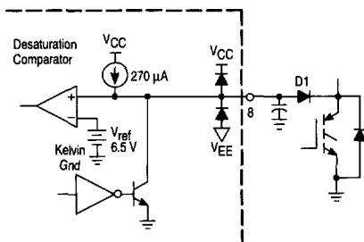
Figure 33. Desaturation Detection
