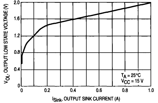
Figure 6. Drive Output Low State Voltage versus Sink Current
