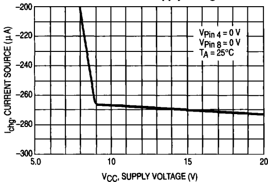
Figure 20. Fault Blanking/Desaturation Current Source versus Supply Voltage
