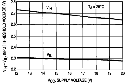
Figure 4. Input Threshold Voltage versus Supply Voltage
