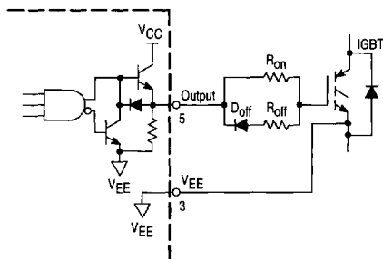
Figure 31. Using Separate Resistors for Turn-On and Turn-Off
