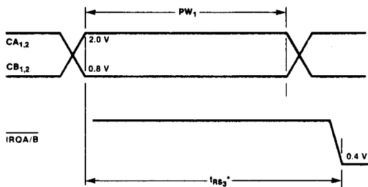
Fig. 16 Interrupt Pulse Width and \overline{IRQ} Response
