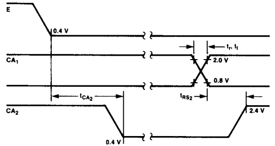
Fig. 12 Peripheral CMOS Data Delay Times (Write Mode; CRA-5 = CRA-3 = 1; CRA-4 = 0)
