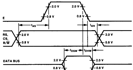
Fig. 4 Bus Timing Characteristics (Write to PIA)
