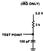
Fig. 8 NMOS Equivalent Test Load
