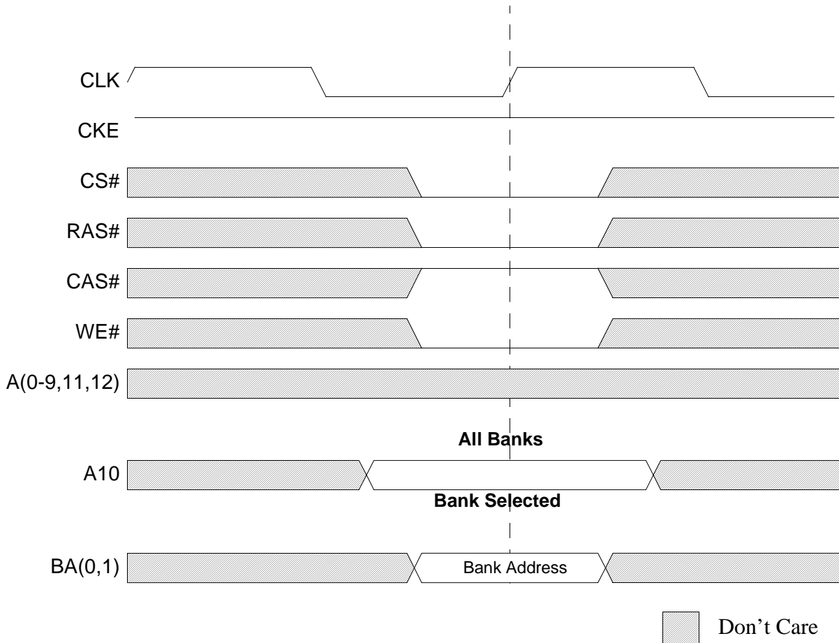
Figure 23: PRECHARGE Command
