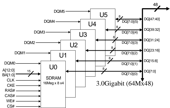
Figure 1. Block Diagrams
