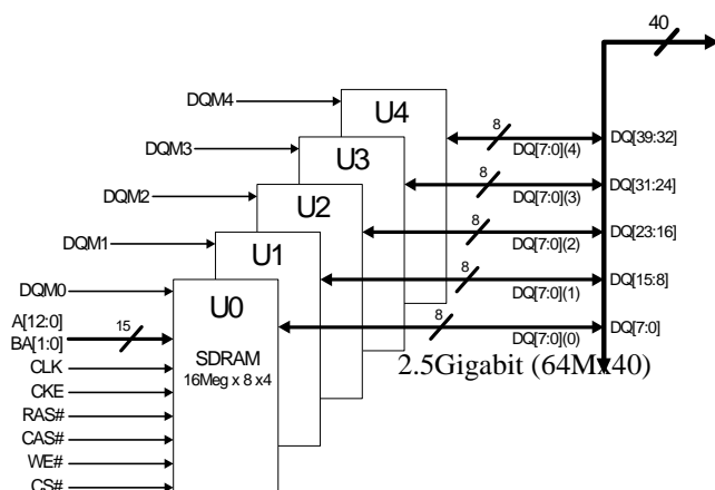
Figure 1. Block Diagrams
