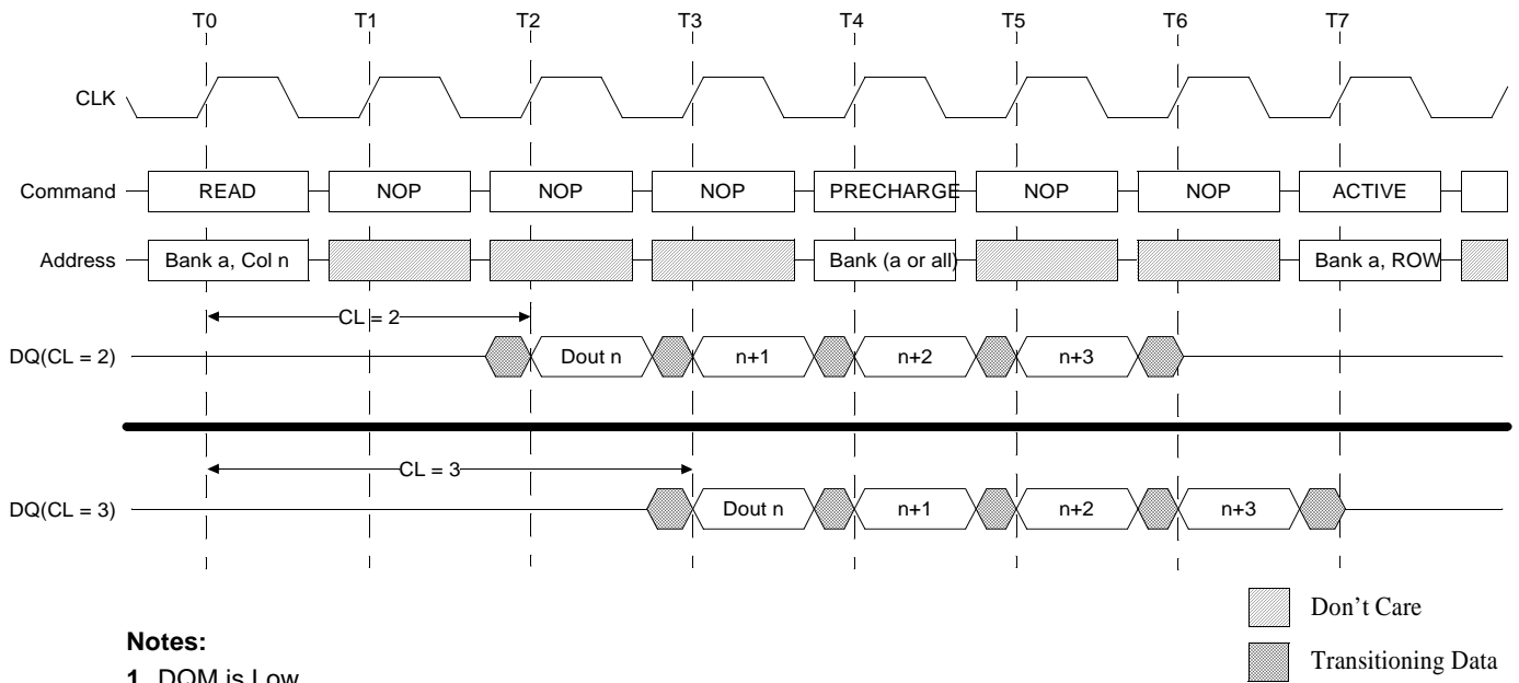
Figure 14: READ-to-PRECHARGE
