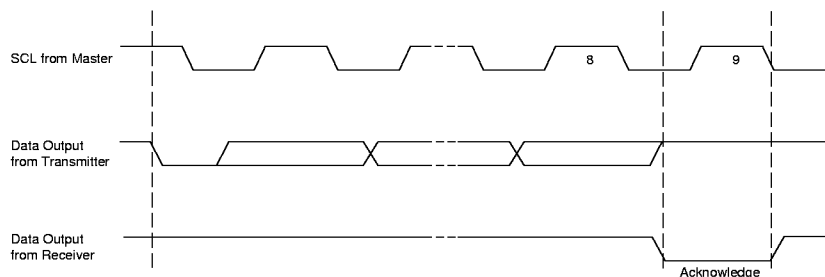
Figure 3 ACKNOWLEDGE RESPONSE FROM RECEIVER
