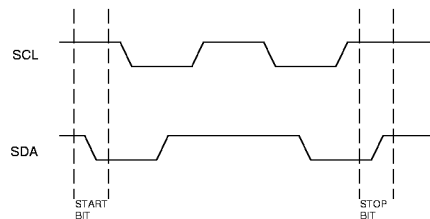
Figure 2 DEFINITION OF START AND STOP
