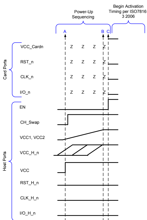
Figure 15. Power-Up Sequencing
