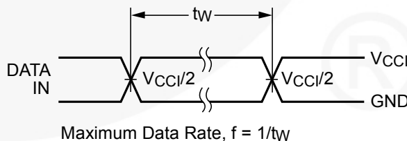
Figure 7. Maximum Data Rate
