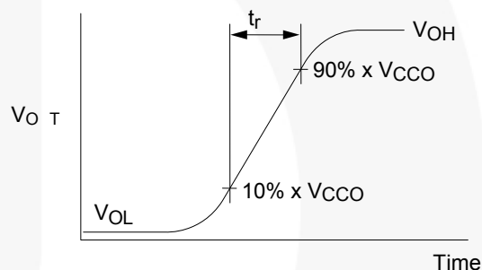
Figure 5. Active Output Rise Time
