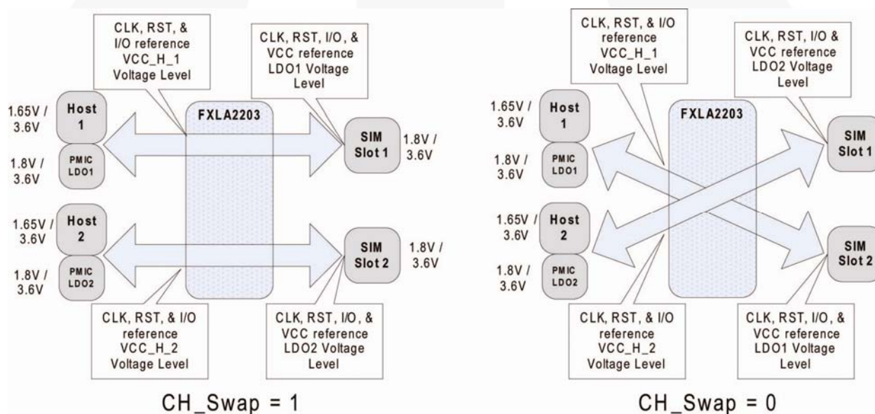
Figure 10. Voltage Translation
