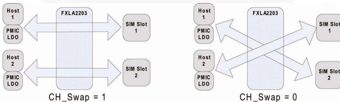
Figure 9. CH_Swap
