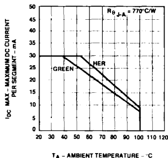
Figure 12. Maximum Allowable DC Current vs. Ambient Temperature.
