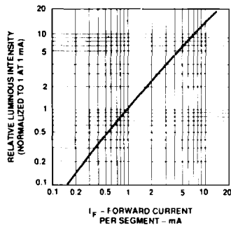
Figure 8. Relative Luminous Intensity vs. DC Forward Current.
