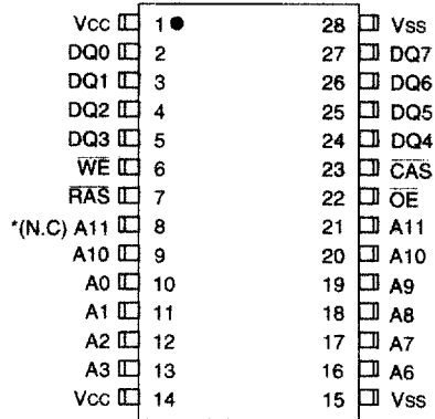
28Pin Plastic TSOP-II (300mil)
