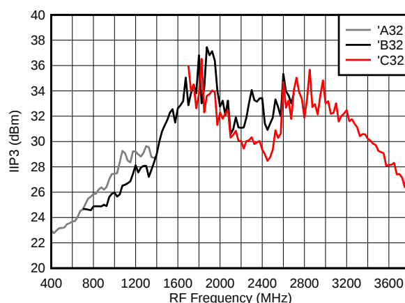
IIP3 Performance Across Frequency
