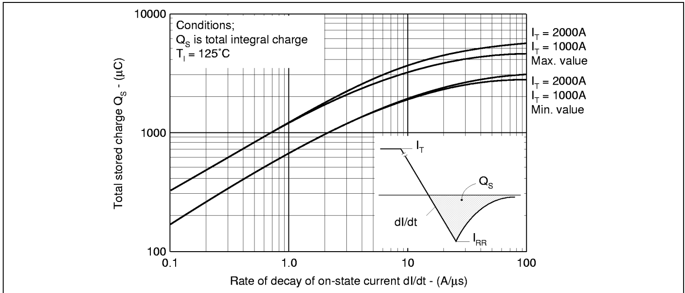
Fig.3 Stored charge
