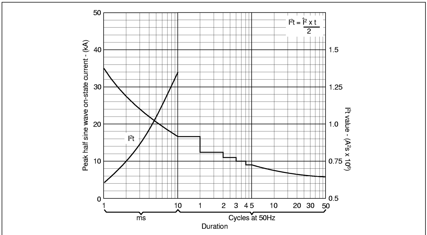
Fig.6 Surge (non-repetitive) on-state current vs time (with 50% V_{RRM} at T_{case} = 125^\circ\text{C} )
