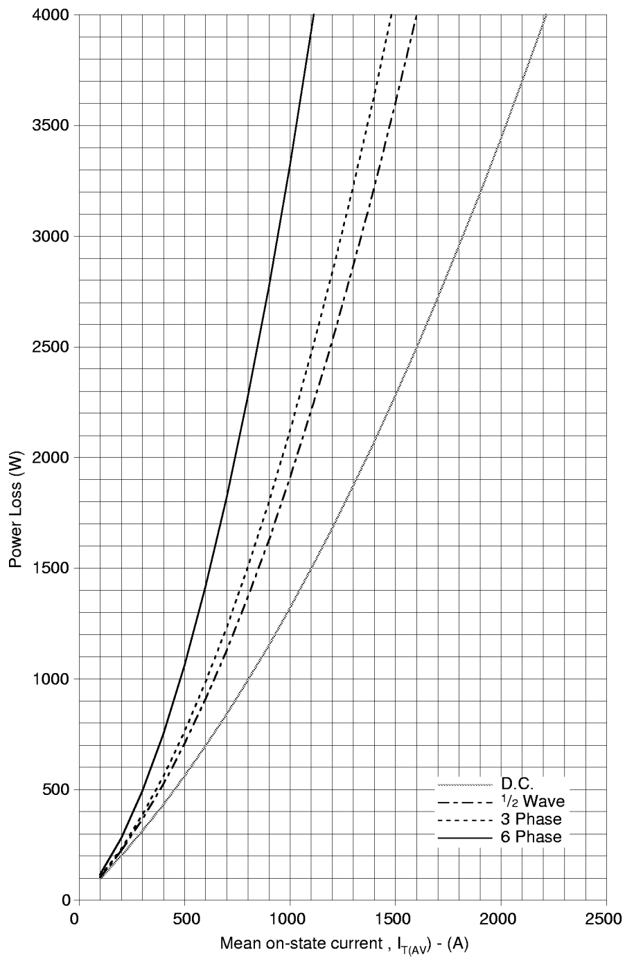
Fig.2 Dissipation curves
