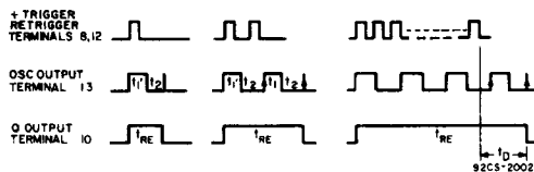
Fig. 29 - Retrigger-mode waveforms.
