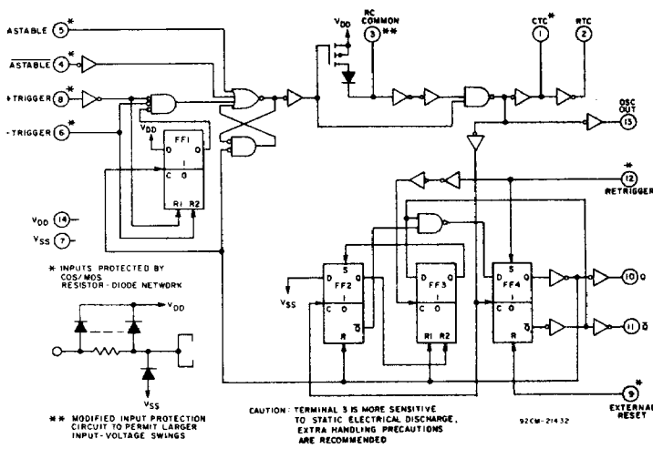
Fig. 9 - CD4047A logic diagram.
