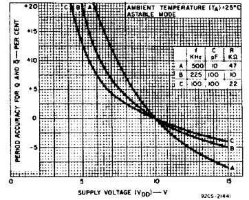
Fig. 10 - Typical Q-and-Q-bar high accuracy vs supply voltage (high frequency).
