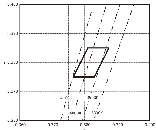
4 000K Chromaticity Diagram
