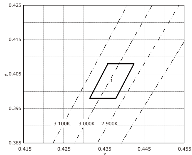
3 000K Chromaticity Diagram
