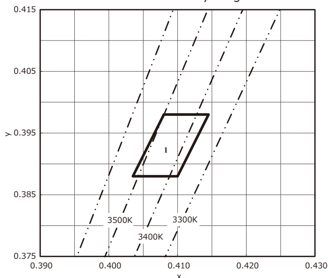
3 500K Chromaticity Diagram
