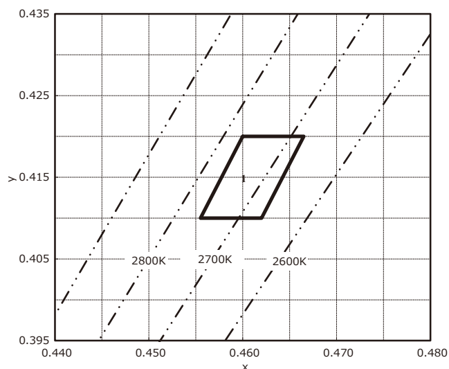
2 700K Chromaticity Diagram
