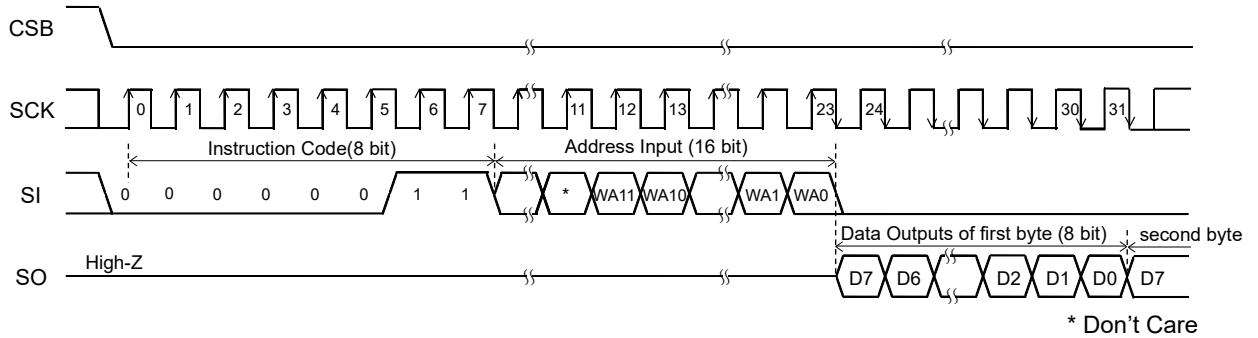
Figure 41. Read Command
