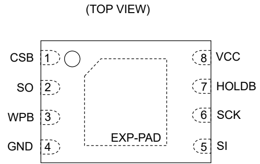
Figure 3-(b). Pin Configuration (VSON008X2030)
