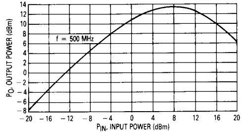
Figure 13. Output Power versus Input Power
