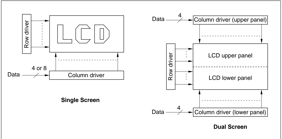
Figure 22 Hardware Configuration According to Screen Format
