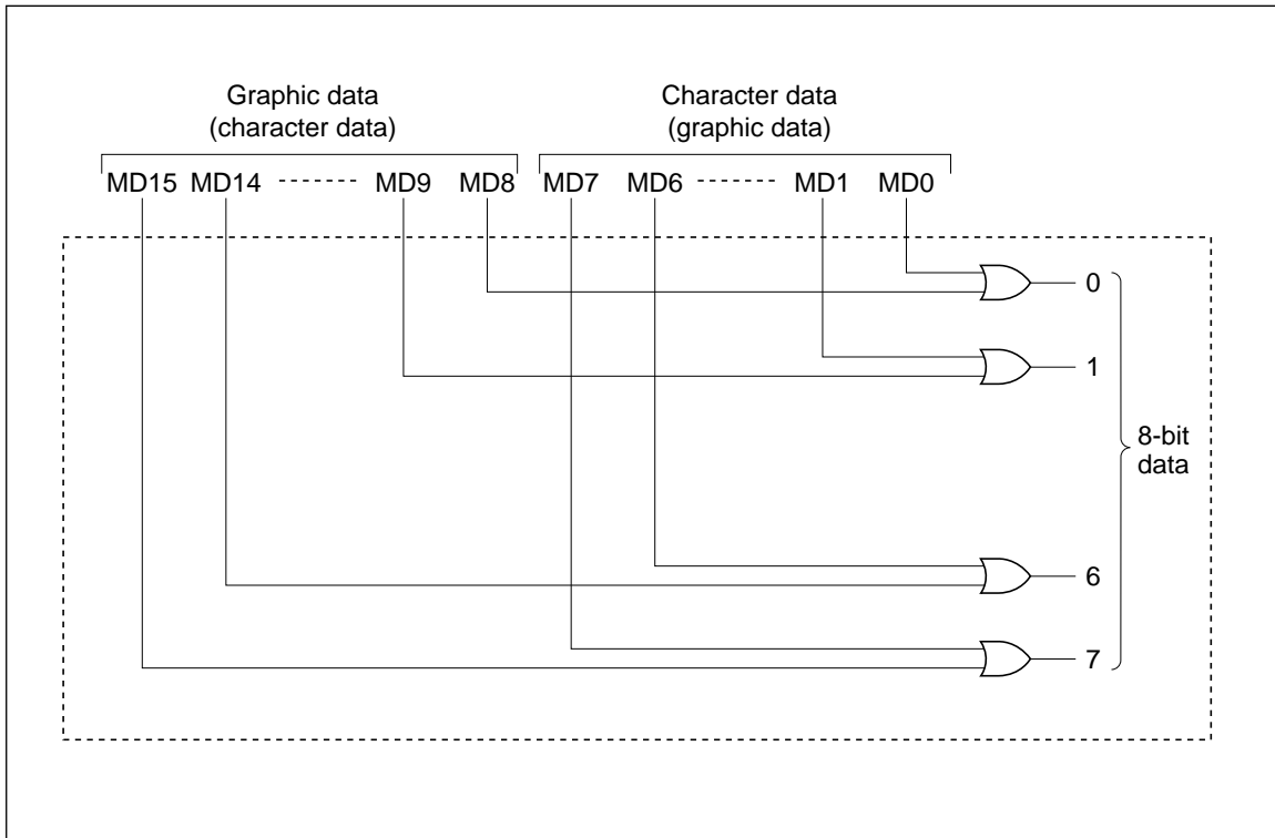
Figure 19 OR Function
