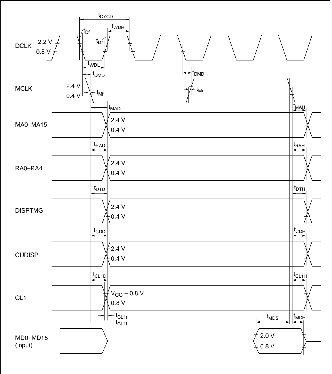
Figure 39 Memory Interface
