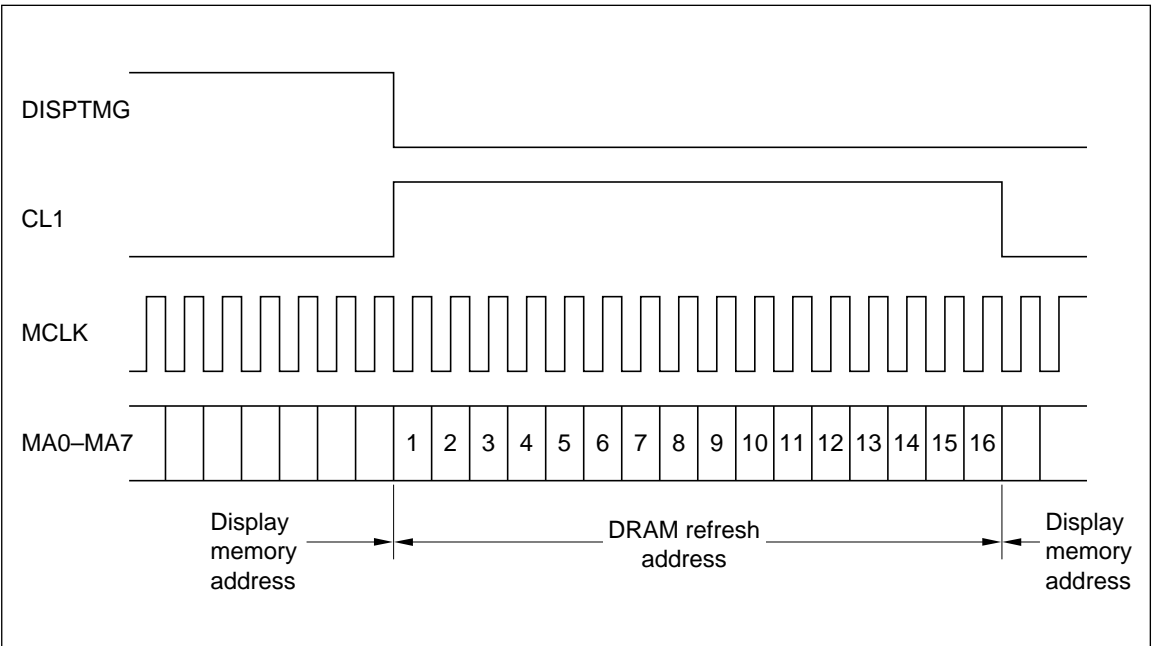
Figure 20 DRAM Refresh Address Output
