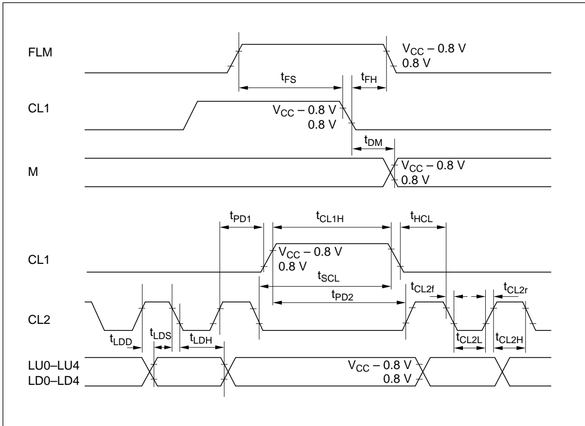
Figure 41 LCD Interface
