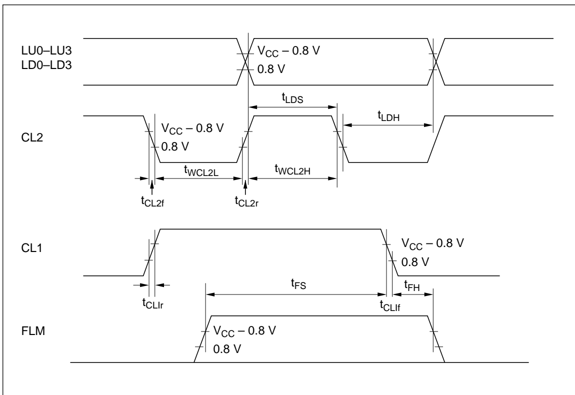
Figure 40 LCD Interface
