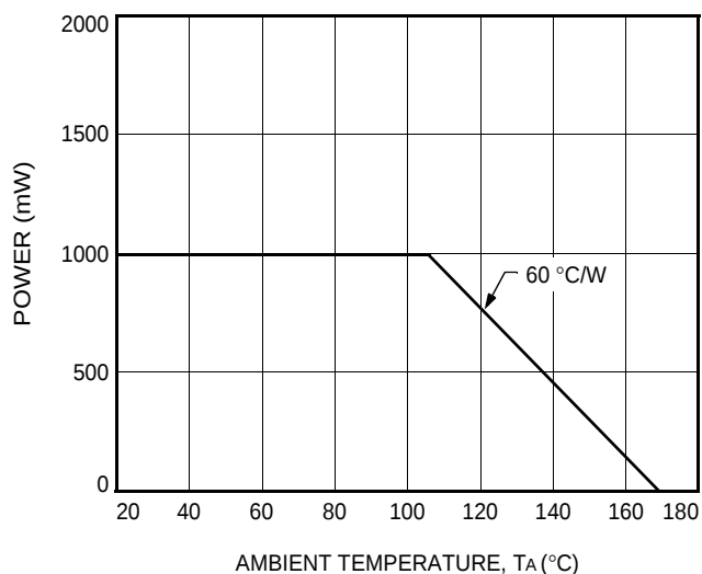
Figure 22. Power Derating
