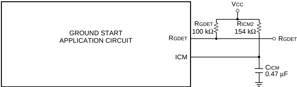
Figure 11. Basic Loop Start Application Circuit Using T7504 Type Codec
