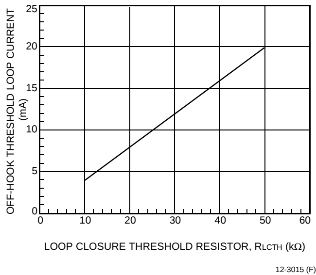
Figure 17. Loop Closure Program Resistor Selection
