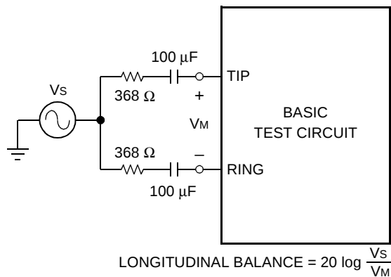
Figure 5. Longitudinal Balance
