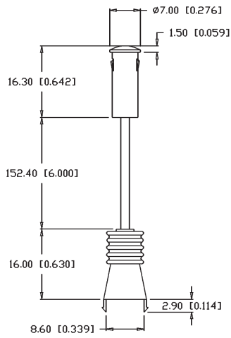
Figure 49 Part # LPI-C011701S-150
